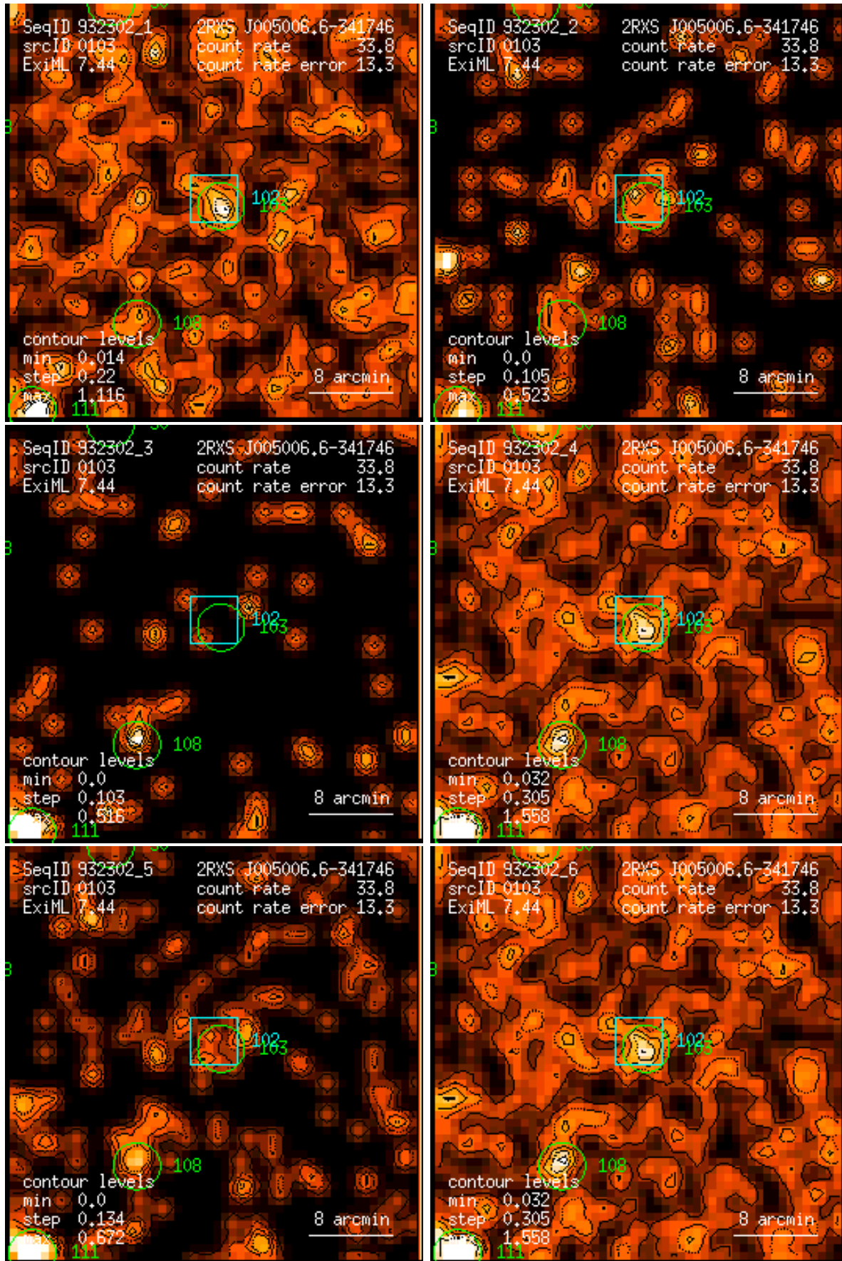
Figure 103: RASS 932302: detection 0103: band rate images, Gaussian filter: (1) PSPC channels 11 – 41, (2) 52 – 90, (3) 91 – 201, (4) 11 – 235, (5) 52 – 201, (6) 11 – 201. Broad band rates in counts/ks. Band rate contour levels in counts/ks/arcmin 2 .
