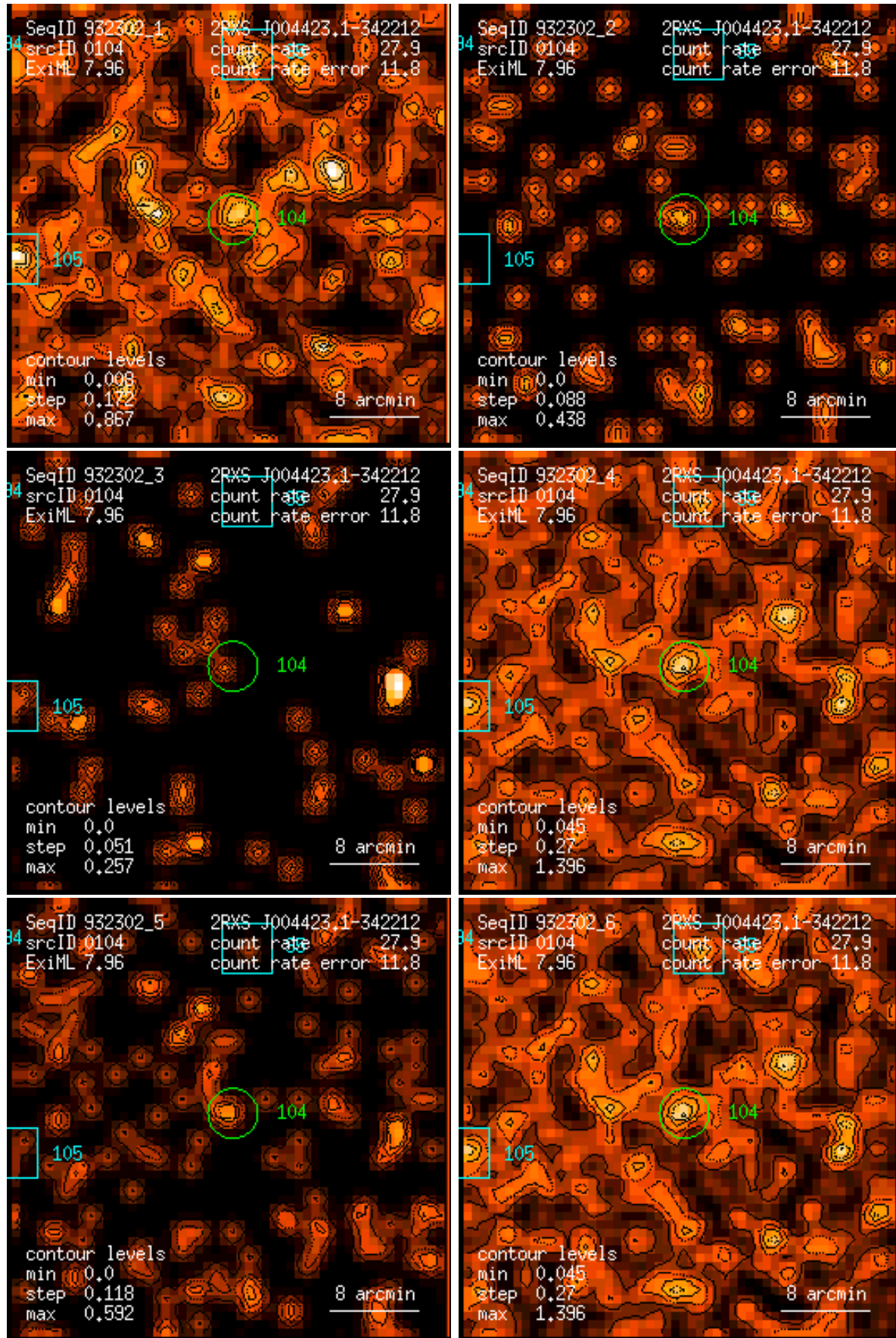
Figure 104: RASS 932302: detection 0104: band rate images, Gaussian filter: (1) PSPC channels 11 – 41, (2) 52 – 90, (3) 91 – 201, (4) 11 – 235, (5) 52 – 201, (6) 11 – 201. Broad band rates in counts/ks. Band rate contour levels in counts/ks/arcmin 2 .
