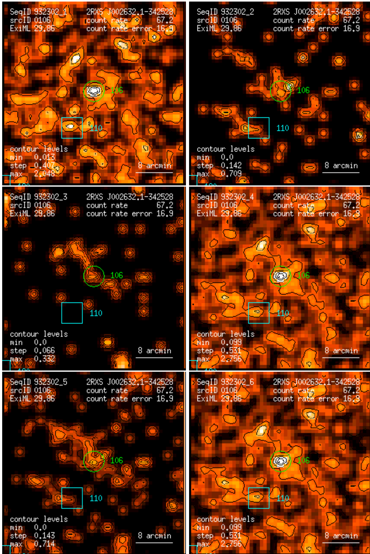
Figure 106: RASS 932302: detection 0106: band rate images, Gaussian filter: (1) PSPC channels 11 – 41, (2) 52 – 90, (3) 91 – 201, (4) 11 – 235, (5) 52 – 201, (6) 11 – 201. Broad band rates in counts/ks. Band rate contour levels in counts/ks/arcmin 2 .
