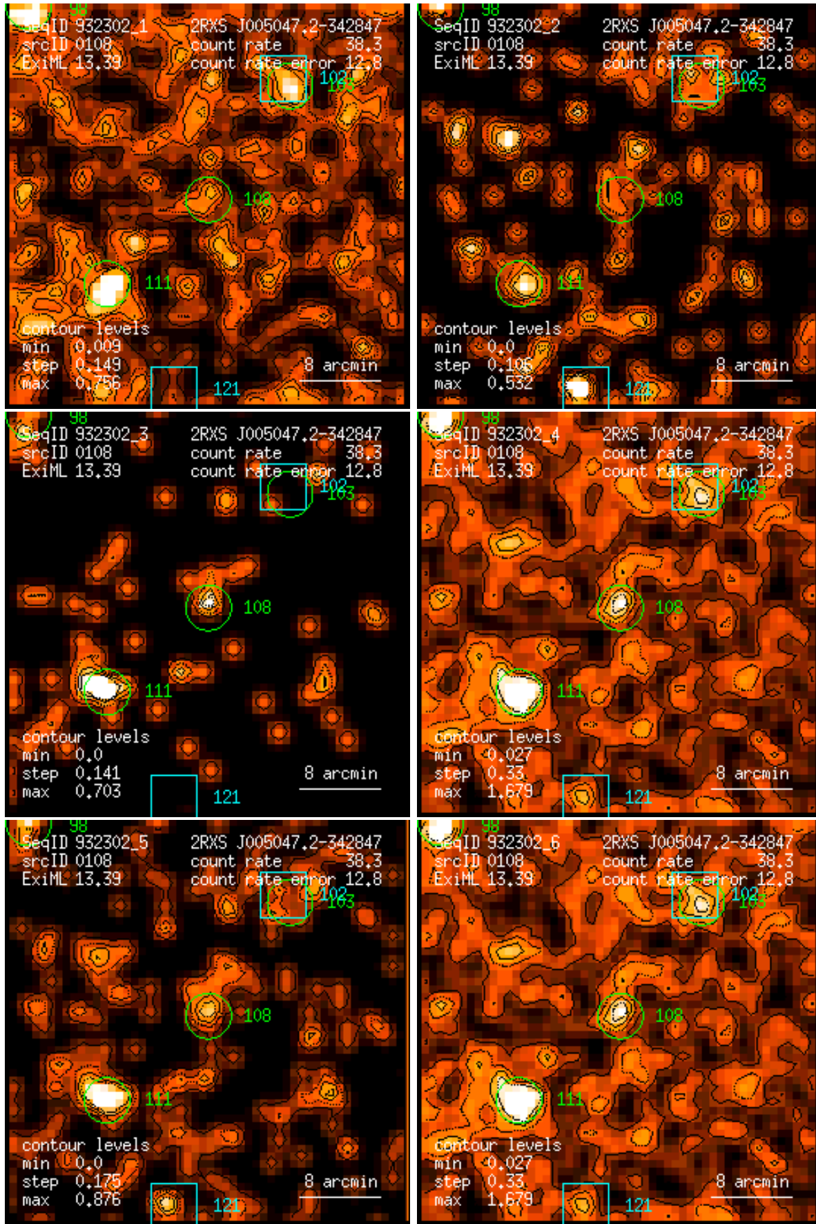
Figure 108: RASS 932302: detection 0108: band rate images, Gaussian filter: (1) PSPC channels 11 – 41, (2) 52 – 90, (3) 91 – 201, (4) 11 – 235, (5) 52 – 201, (6) 11 – 201. Broad band rates in counts/ks. Band rate contour levels in counts/ks/arcmin 2 .
