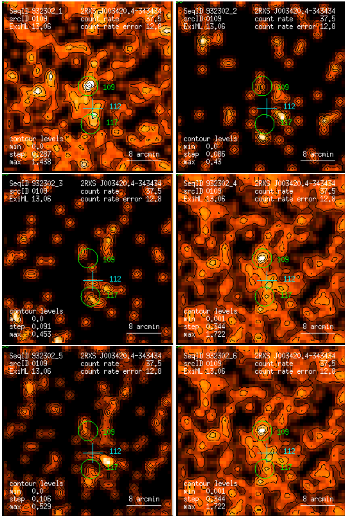
Figure 109: RASS 932302: detection 0109: band rate images, Gaussian filter: (1) PSPC channels 11 – 41, (2) 52 – 90, (3) 91 – 201, (4) 11 – 235, (5) 52 – 201, (6) 11 – 201. Broad band rates in counts/ks. Band rate contour levels in counts/ks/arcmin 2 .
