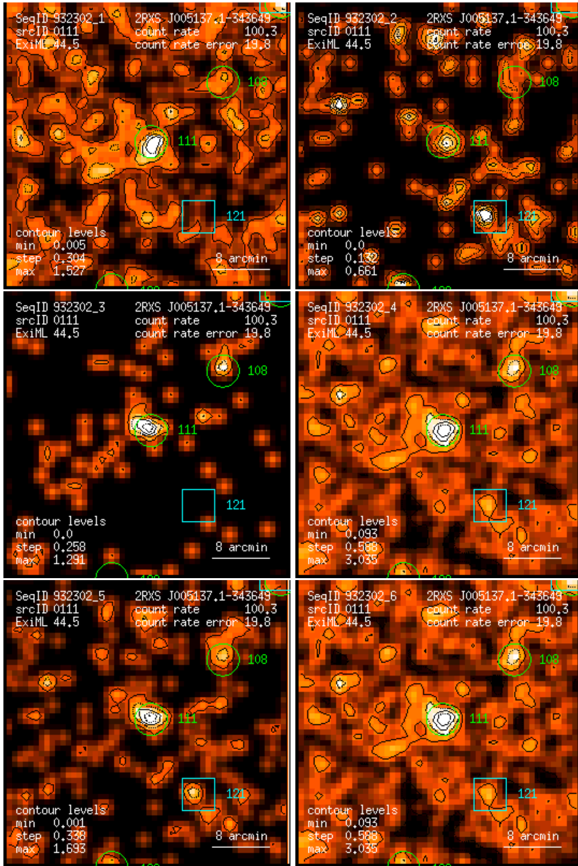
Figure 111: RASS 932302: detection 0111: band rate images, Gaussian filter: (1) PSPC channels 11 – 41, (2) 52 – 90, (3) 91 – 201, (4) 11 – 235, (5) 52 – 201, (6) 11 – 201. Broad band rates in counts/ks. Band rate contour levels in counts/ks/arcmin 2 .
