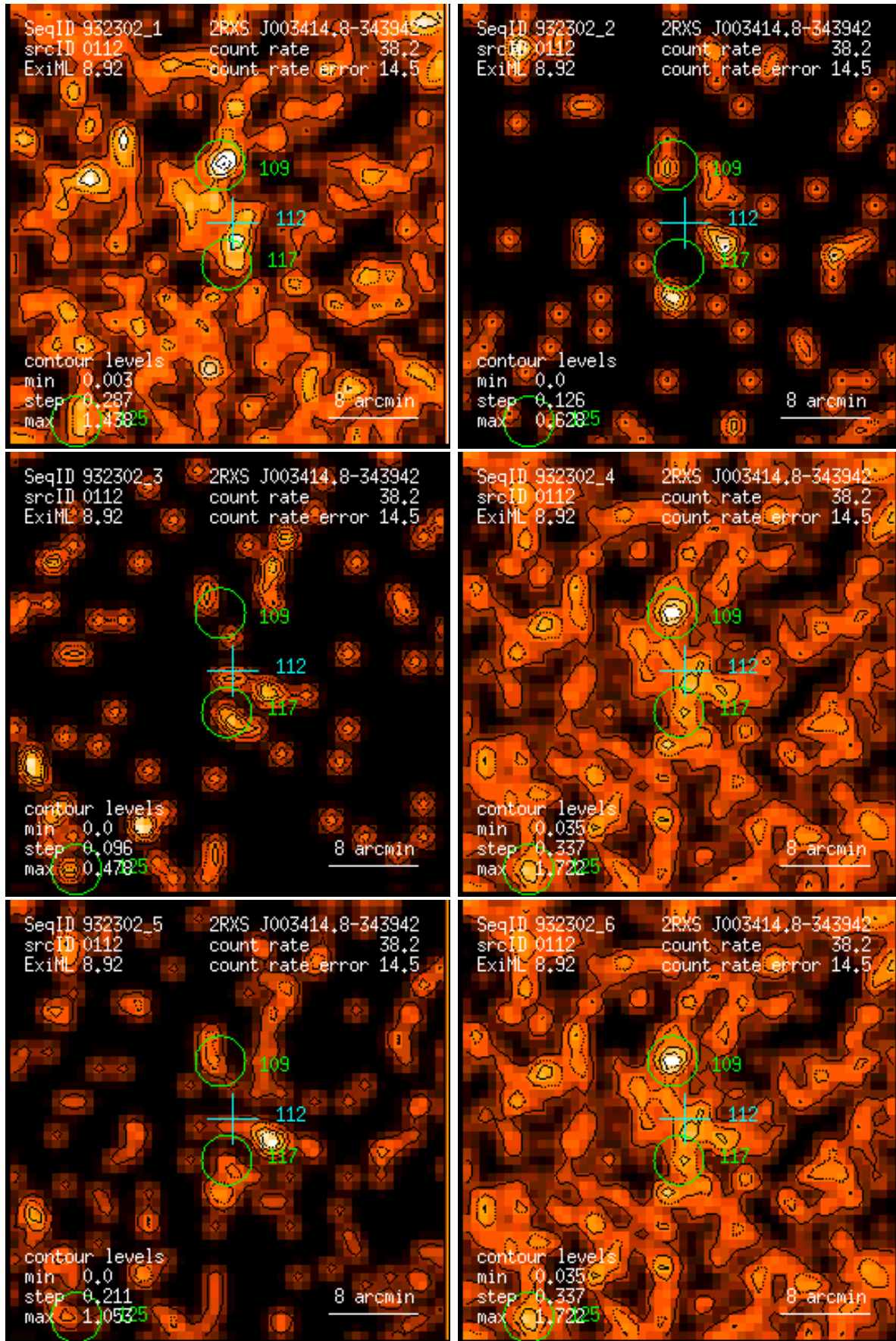
Figure 112: RASS 932302: detection 0112: band rate images, Gaussian filter: (1) PSPC channels 11 – 41, (2) 52 – 90, (3) 91 – 201, (4) 11 – 235, (5) 52 – 201, (6) 11 – 201. Broad band rates in counts/ks. Band rate contour levels in counts/ks/arcmin 2 .
