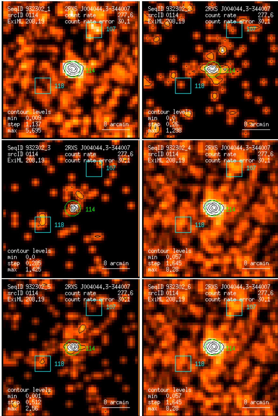
Figure 114: RASS 932302: detection 0114: band rate images, Gaussian filter: (1) PSPC channels 11 – 41, (2) 52 – 90, (3) 91 – 201, (4) 11 – 235, (5) 52 – 201, (6) 11 – 201. Broad band rates in counts/ks. Band rate contour levels in counts/ks/arcmin 2 .
