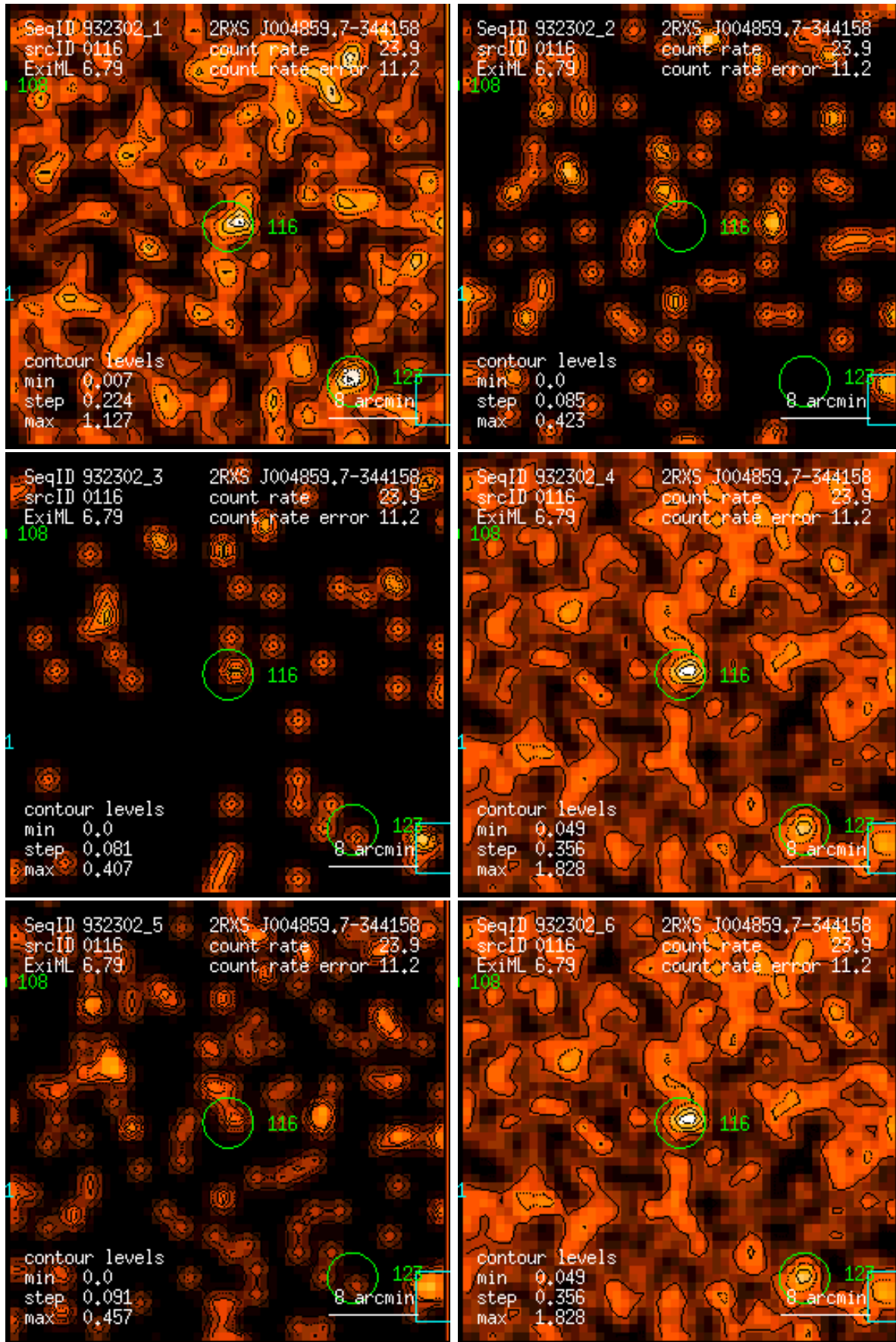
Figure 116: RASS 932302: detection 0116: band rate images, Gaussian filter: (1) PSPC channels 11 – 41, (2) 52 – 90, (3) 91 – 201, (4) 11 – 235, (5) 52 – 201, (6) 11 – 201. Broad band rates in counts/ks. Band rate contour levels in counts/ks/arcmin 2 .
