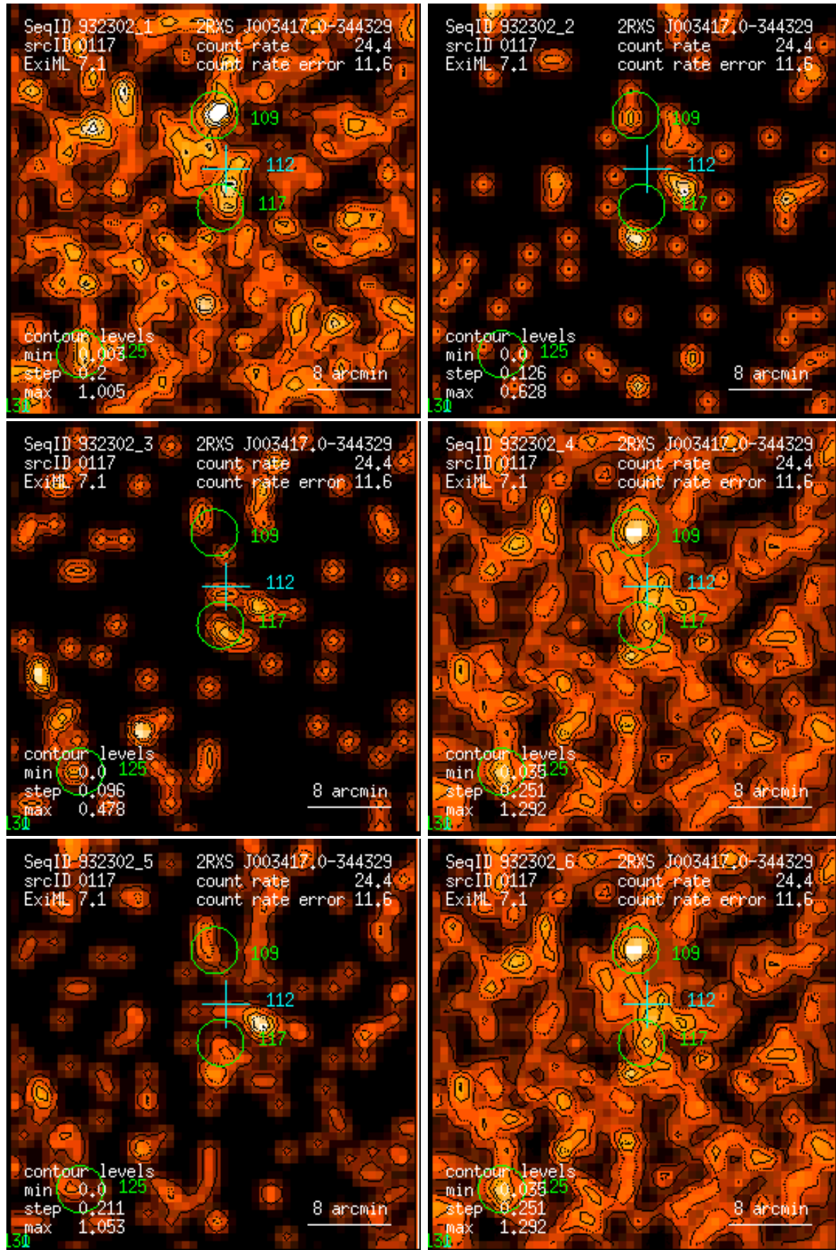
Figure 117: RASS 932302: detection 0117: band rate images, Gaussian filter: (1) PSPC channels 11 – 41, (2) 52 – 90, (3) 91 – 201, (4) 11 – 235, (5) 52 – 201, (6) 11 – 201. Broad band rates in counts/ks. Band rate contour levels in counts/ks/arcmin 2 .
