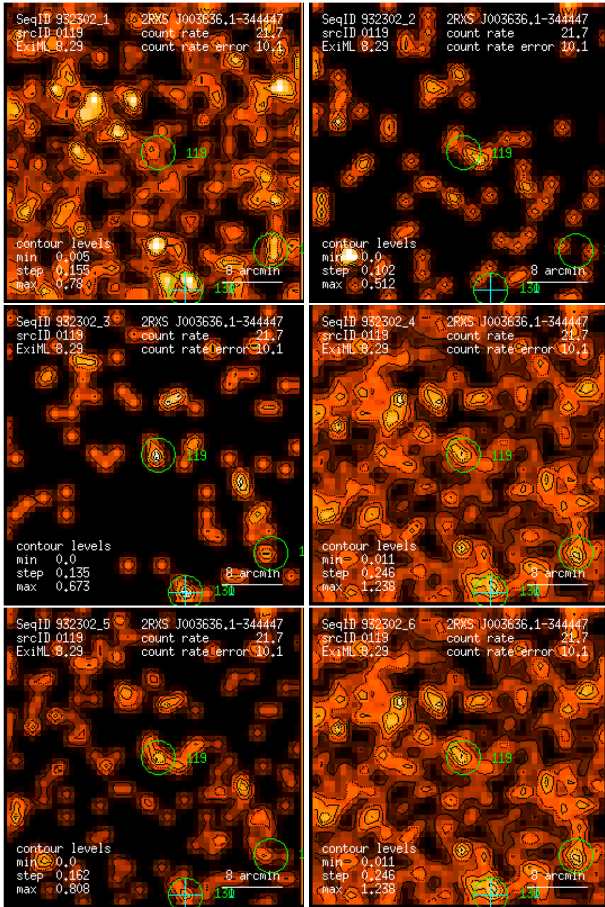
Figure 119: RASS 932302: detection 0119: band rate images, Gaussian filter: (1) PSPC channels 11 – 41, (2) 52 – 90, (3) 91 – 201, (4) 11 – 235, (5) 52 – 201, (6) 11 – 201. Broad band rates in counts/ks. Band rate contour levels in counts/ks/arcmin 2 .
