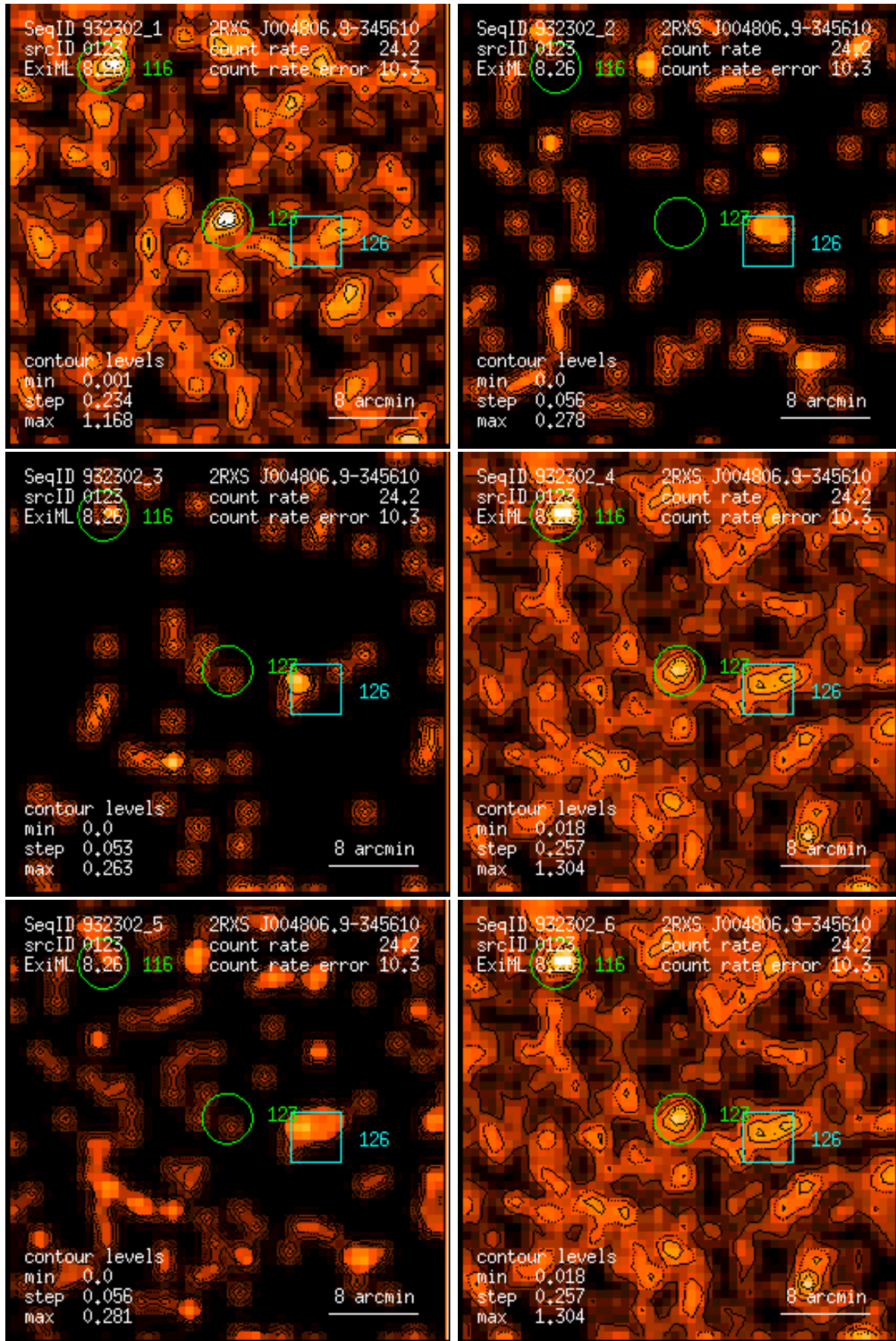
Figure 123: RASS 932302: detection 0123: band rate images, Gaussian filter: (1) PSPC channels 11 – 41, (2) 52 – 90, (3) 91 – 201, (4) 11 – 235, (5) 52 – 201, (6) 11 – 201. Broad band rates in counts/ks. Band rate contour levels in counts/ks/arcmin 2 .
