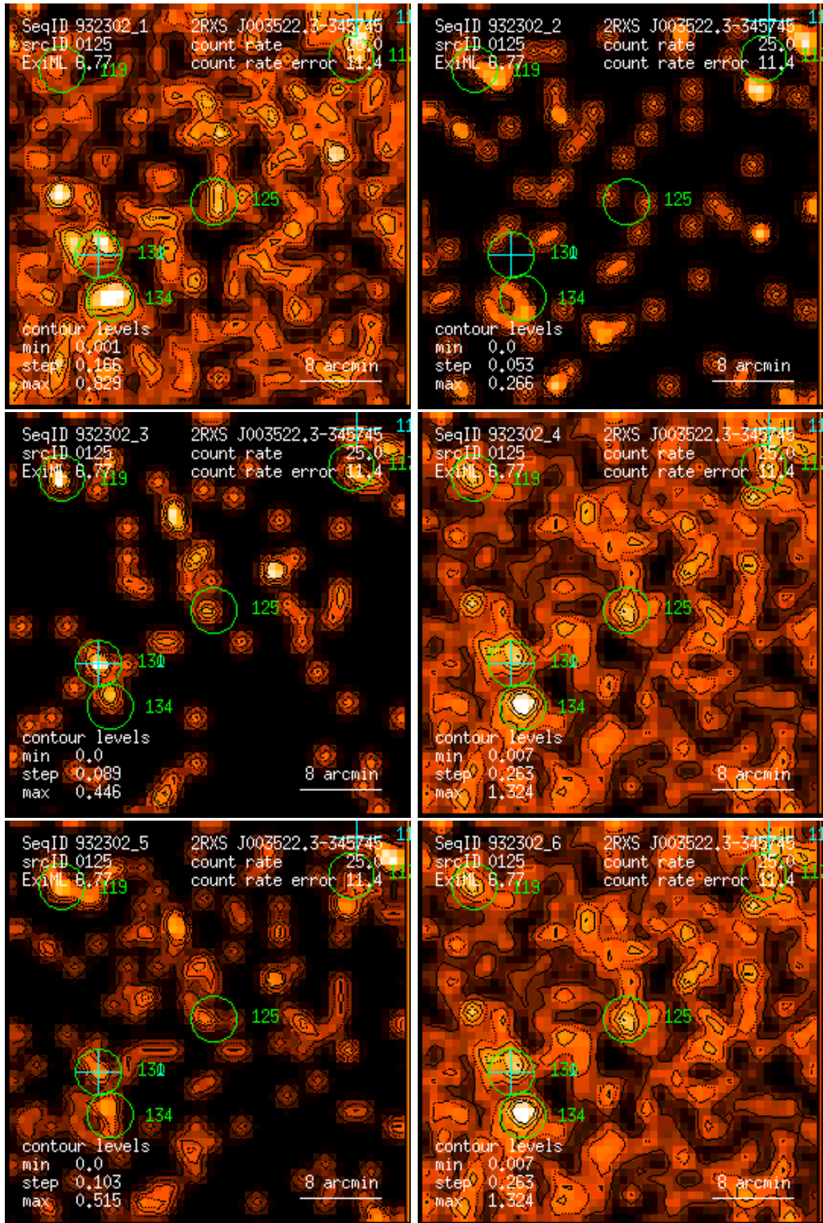
Figure 125: RASS 932302: detection 0125: band rate images, Gaussian filter: (1) PSPC channels 11 – 41, (2) 52 – 90, (3) 91 – 201, (4) 11 – 235, (5) 52 – 201, (6) 11 – 201. Broad band rates in counts/ks. Band rate contour levels in counts/ks/arcmin 2 .
