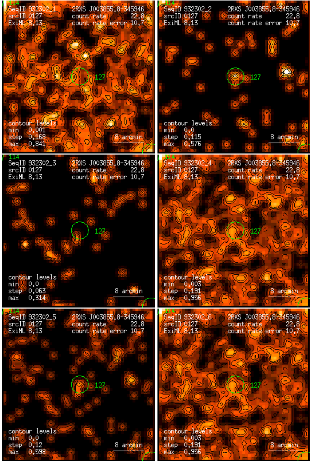
Figure 127: RASS 932302: detection 0127: band rate images, Gaussian filter: (1) PSPC channels 11 – 41, (2) 52 – 90, (3) 91 – 201, (4) 11 – 235, (5) 52 – 201, (6) 11 – 201. Broad band rates in counts/ks. Band rate contour levels in counts/ks/arcmin 2 .
