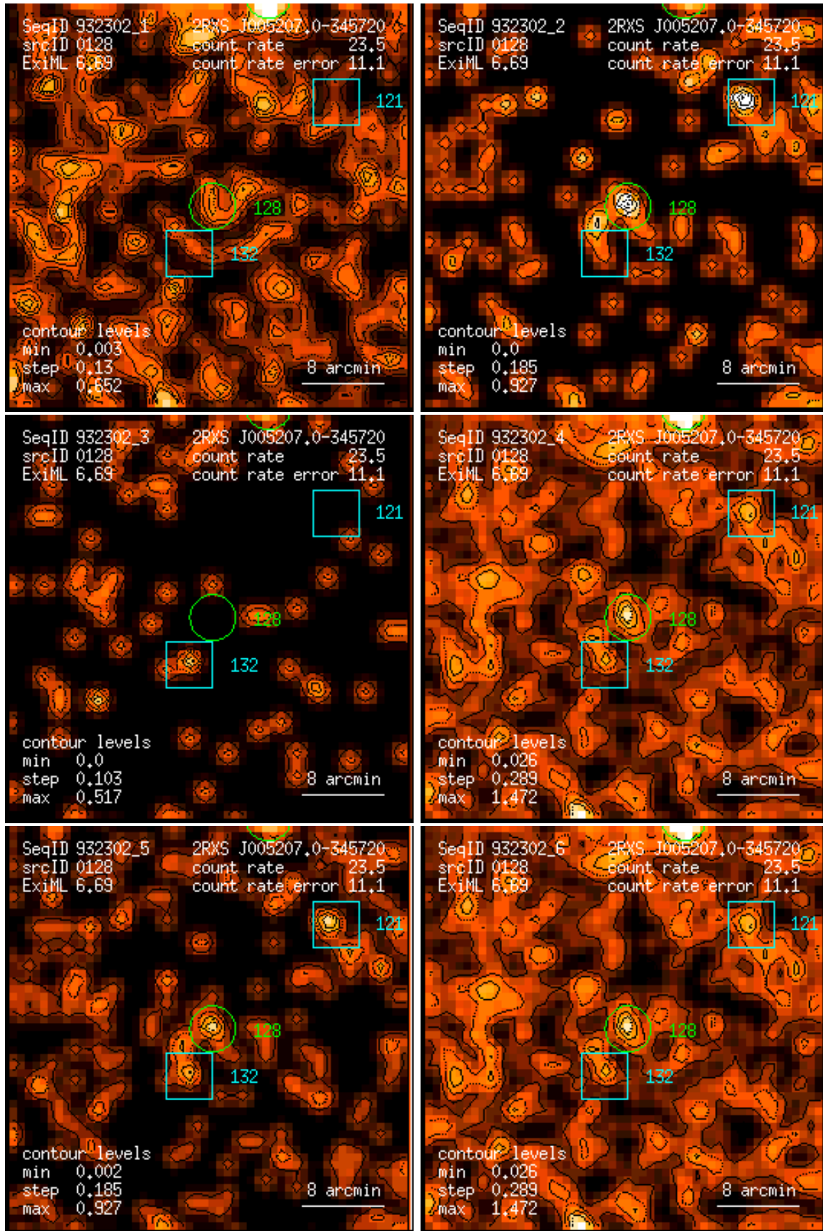
Figure 128: RASS 932302: detection 0128: band rate images, Gaussian filter: (1) PSPC channels 11 – 41, (2) 52 – 90, (3) 91 – 201, (4) 11 – 235, (5) 52 – 201, (6) 11 – 201. Broad band rates in counts/ks. Band rate contour levels in counts/ks/arcmin 2 .
