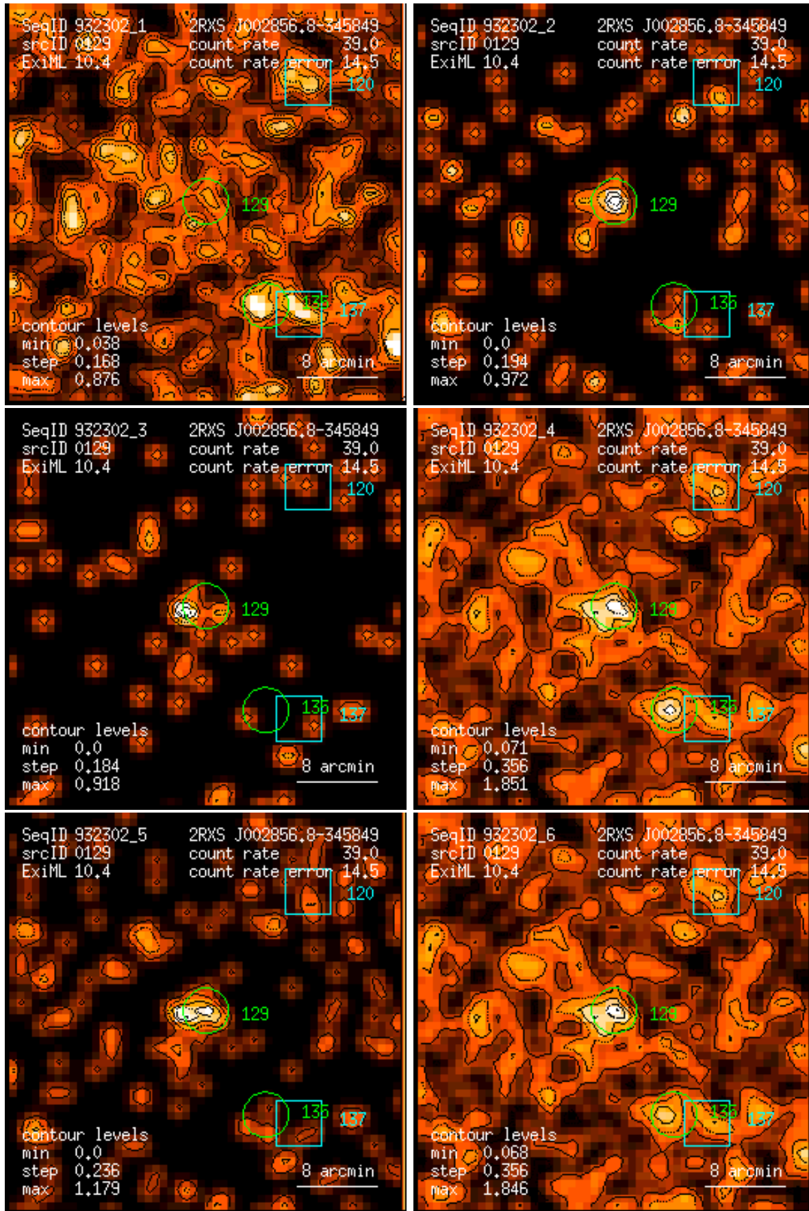
Figure 129: RASS 932302: detection 0129: band rate images, Gaussian filter: (1) PSPC channels 11 – 41, (2) 52 – 90, (3) 91 – 201, (4) 11 – 235, (5) 52 – 201, (6) 11 – 201. Broad band rates in counts/ks. Band rate contour levels in counts/ks/arcmin 2 .
