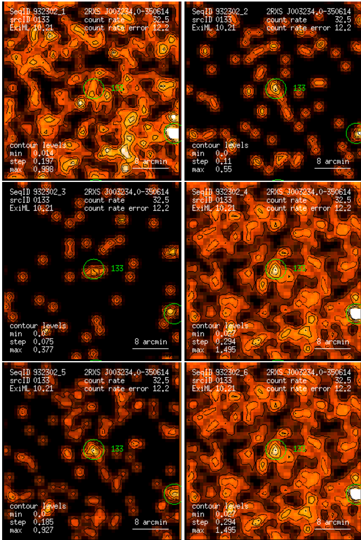
Figure 133: RASS 932302: detection 0133: band rate images, Gaussian filter: (1) PSPC channels 11 – 41, (2) 52 – 90, (3) 91 – 201, (4) 11 – 235, (5) 52 – 201, (6) 11 – 201. Broad band rates in counts/ks. Band rate contour levels in counts/ks/arcmin 2 .
