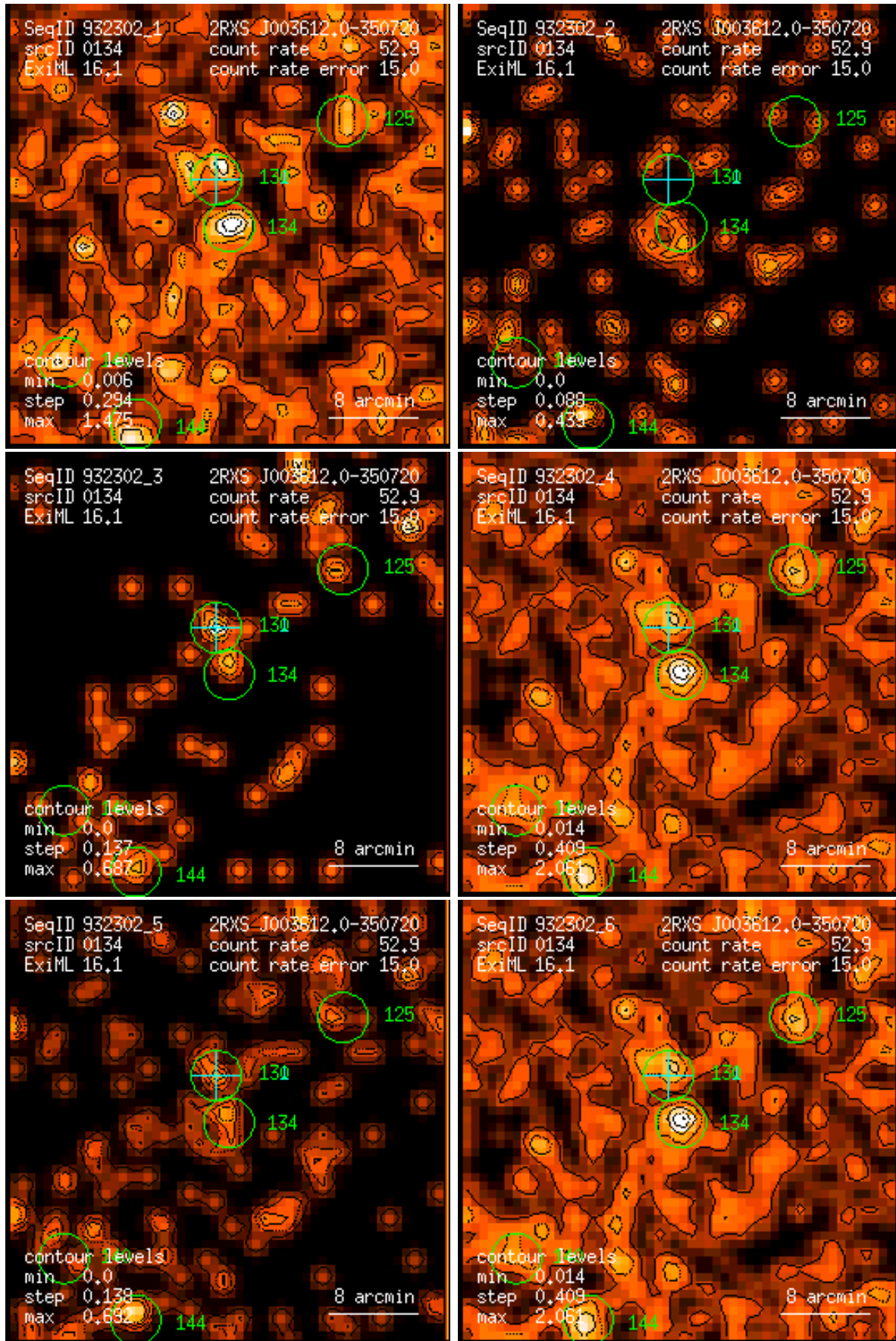
Figure 134: RASS 932302: detection 0134: band rate images, Gaussian filter: (1) PSPC channels 11 – 41, (2) 52 – 90, (3) 91 – 201, (4) 11 – 235, (5) 52 – 201, (6) 11 – 201. Broad band rates in counts/ks. Band rate contour levels in counts/ks/arcmin 2 .
