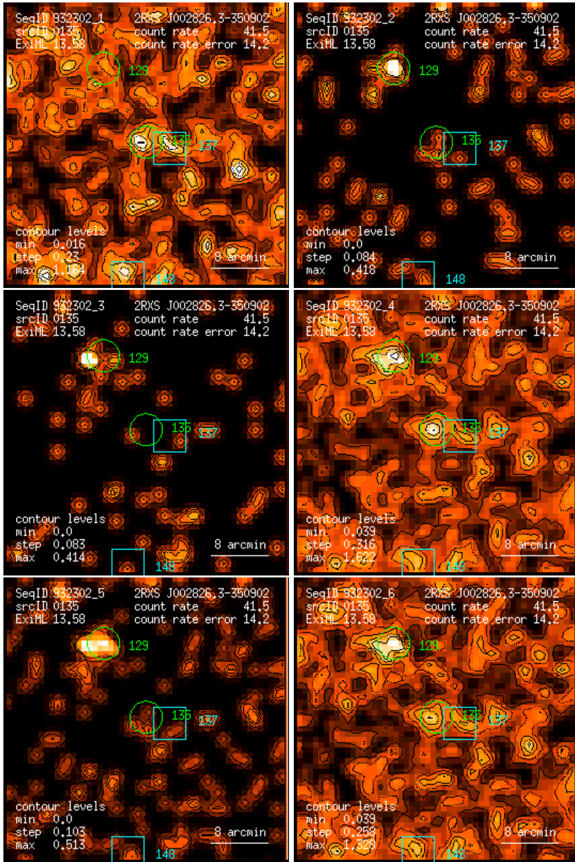
Figure 135: RASS 932302: detection 0135: band rate images, Gaussian filter: (1) PSPC channels 11 – 41, (2) 52 – 90, (3) 91 – 201, (4) 11 – 235, (5) 52 – 201, (6) 11 – 201. Broad band rates in counts/ks. Band rate contour levels in counts/ks/arcmin 2 .
