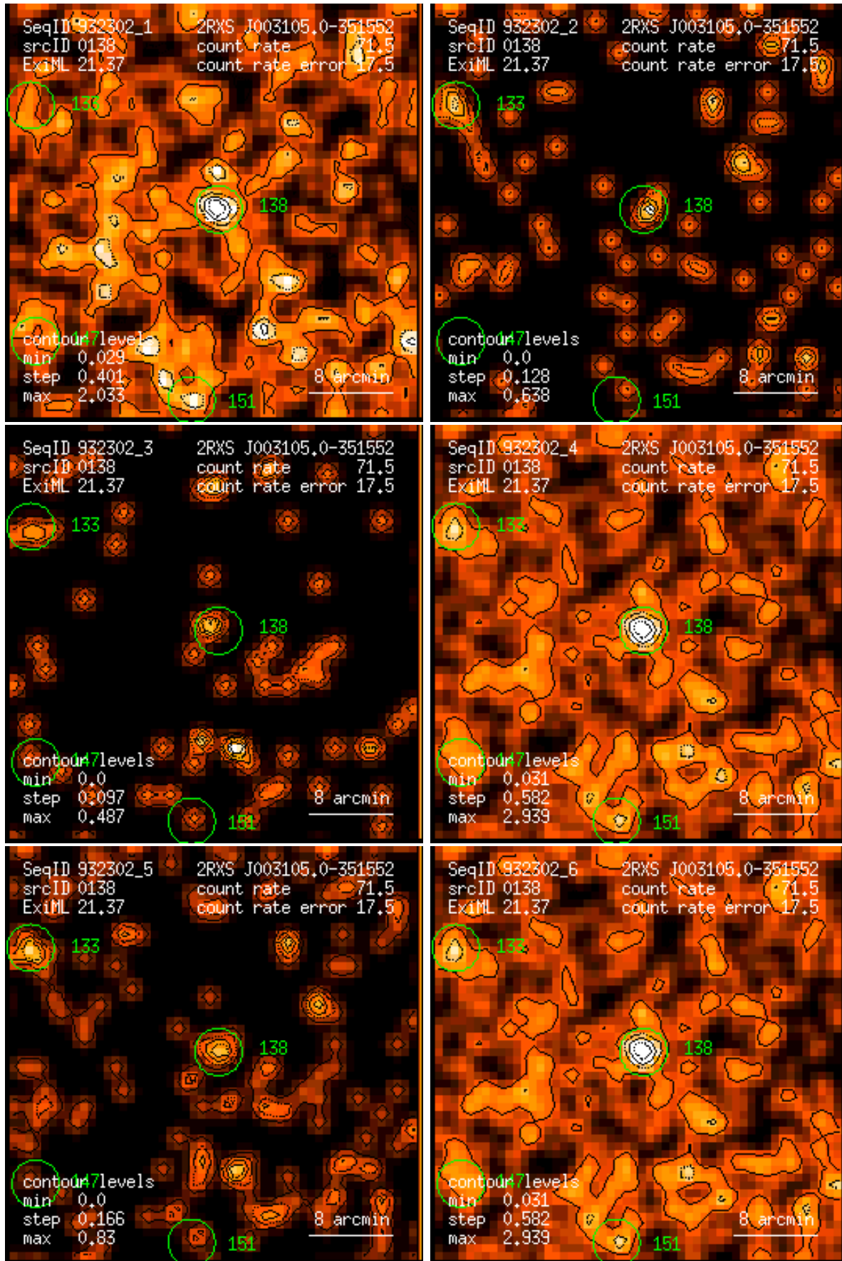
Figure 138: RASS 932302: detection 0138: band rate images, Gaussian filter: (1) PSPC channels 11 – 41, (2) 52 – 90, (3) 91 – 201, (4) 11 – 235, (5) 52 – 201, (6) 11 – 201. Broad band rates in counts/ks. Band rate contour levels in counts/ks/arcmin 2 .
