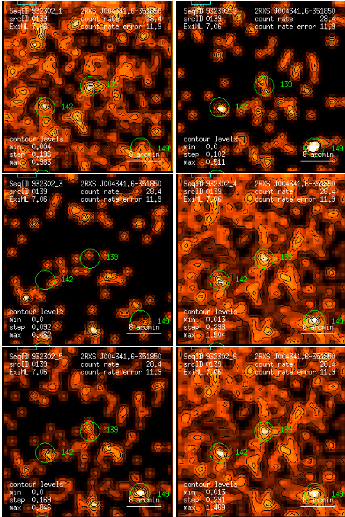
Figure 139: RASS 932302: detection 0139: band rate images, Gaussian filter: (1) PSPC channels 11 – 41, (2) 52 – 90, (3) 91 – 201, (4) 11 – 235, (5) 52 – 201, (6) 11 – 201. Broad band rates in counts/ks. Band rate contour levels in counts/ks/arcmin 2 .
