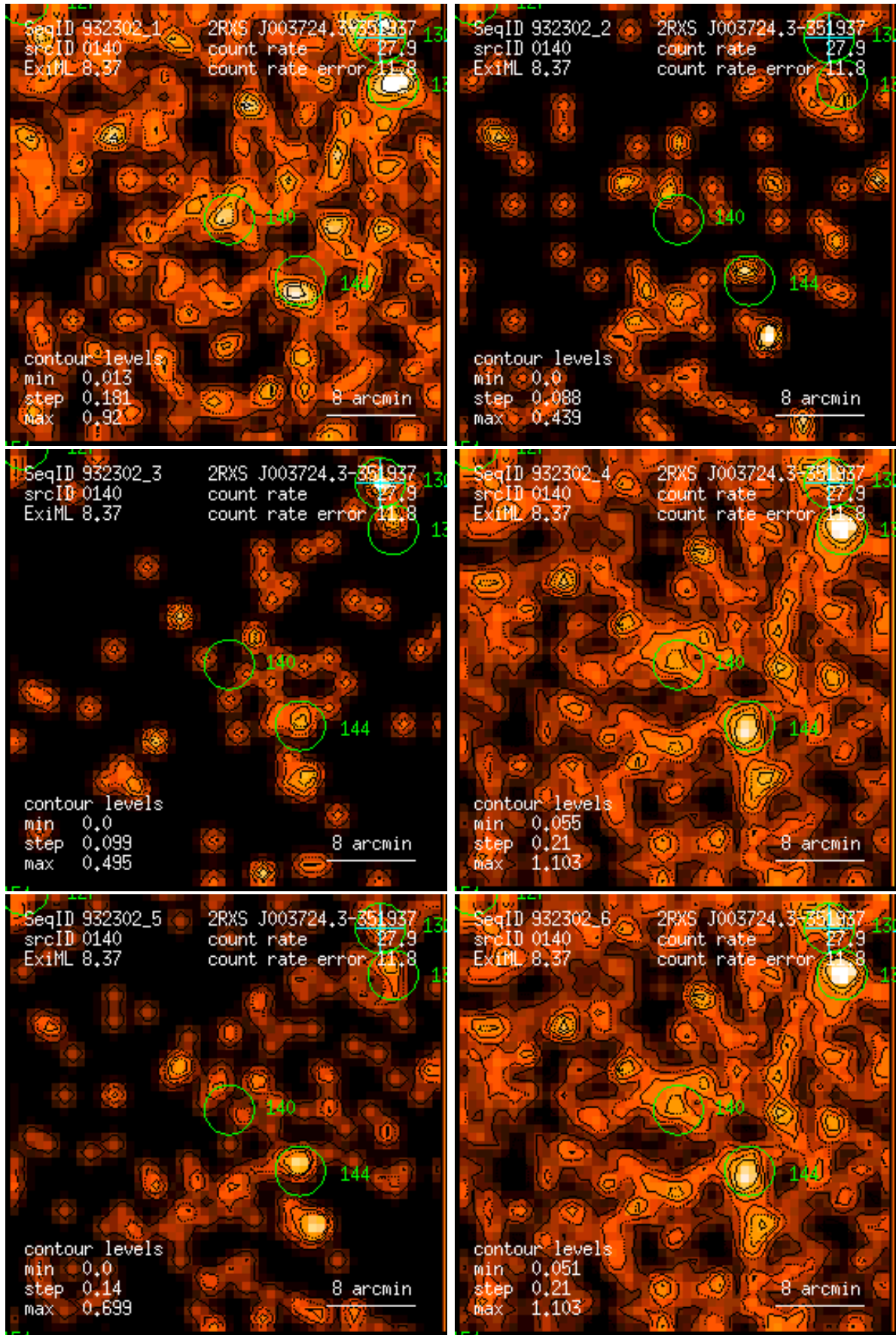
Figure 140: RASS 932302: detection 0140: band rate images, Gaussian filter: (1) PSPC channels 11 – 41, (2) 52 – 90, (3) 91 – 201, (4) 11 – 235, (5) 52 – 201, (6) 11 – 201. Broad band rates in counts/ks. Band rate contour levels in counts/ks/arcmin 2 .
