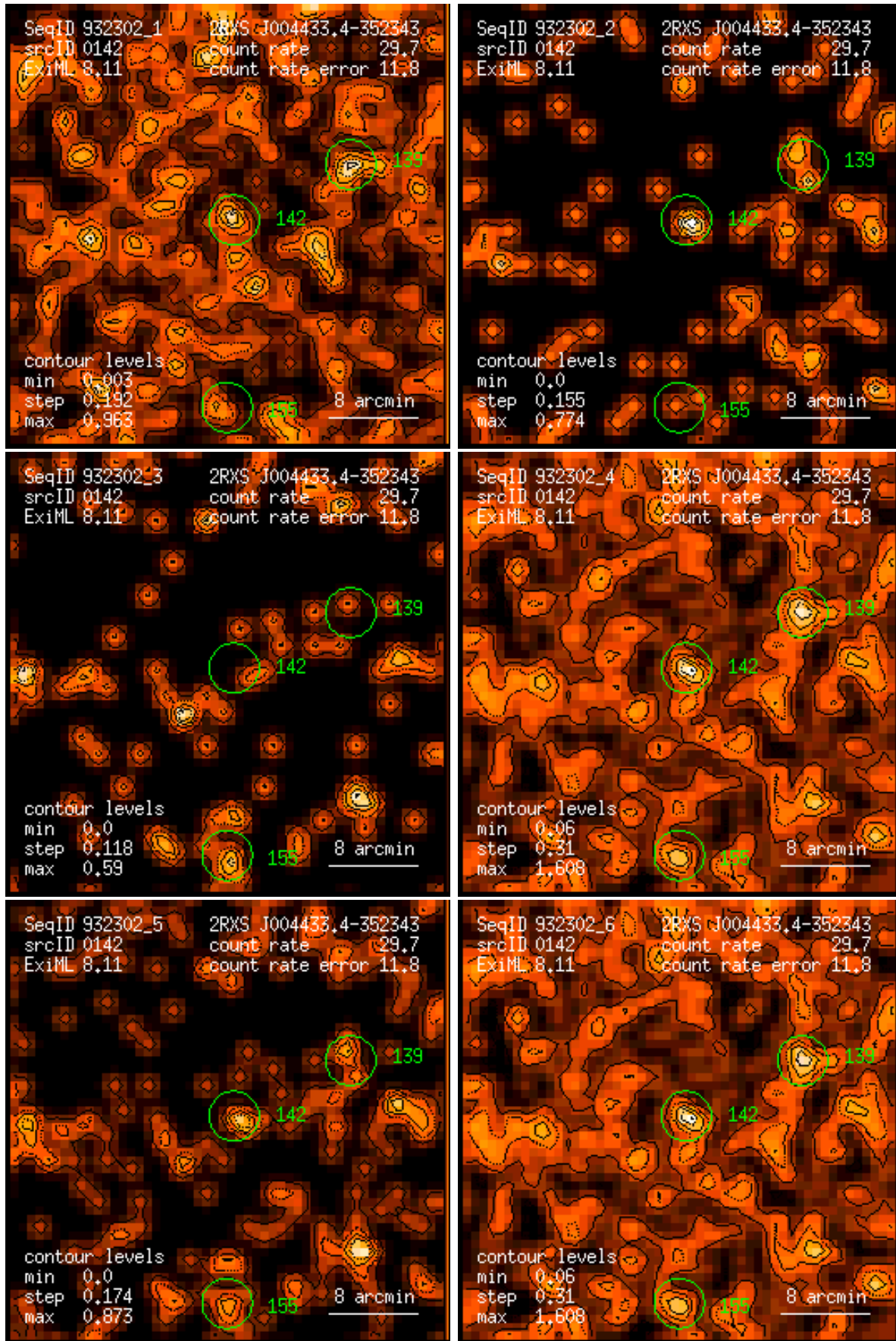
Figure 142: RASS 932302: detection 0142: band rate images, Gaussian filter: (1) PSPC channels 11 – 41, (2) 52 – 90, (3) 91 – 201, (4) 11 – 235, (5) 52 – 201, (6) 11 – 201. Broad band rates in counts/ks. Band rate contour levels in counts/ks/arcmin 2 .
