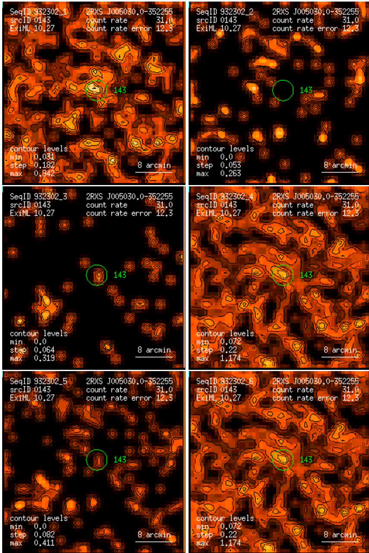
Figure 143: RASS 932302: detection 0143: band rate images, Gaussian filter: (1) PSPC channels 11 – 41, (2) 52 – 90, (3) 91 – 201, (4) 11 – 235, (5) 52 – 201, (6) 11 – 201. Broad band rates in counts/ks. Band rate contour levels in counts/ks/arcmin 2 .
