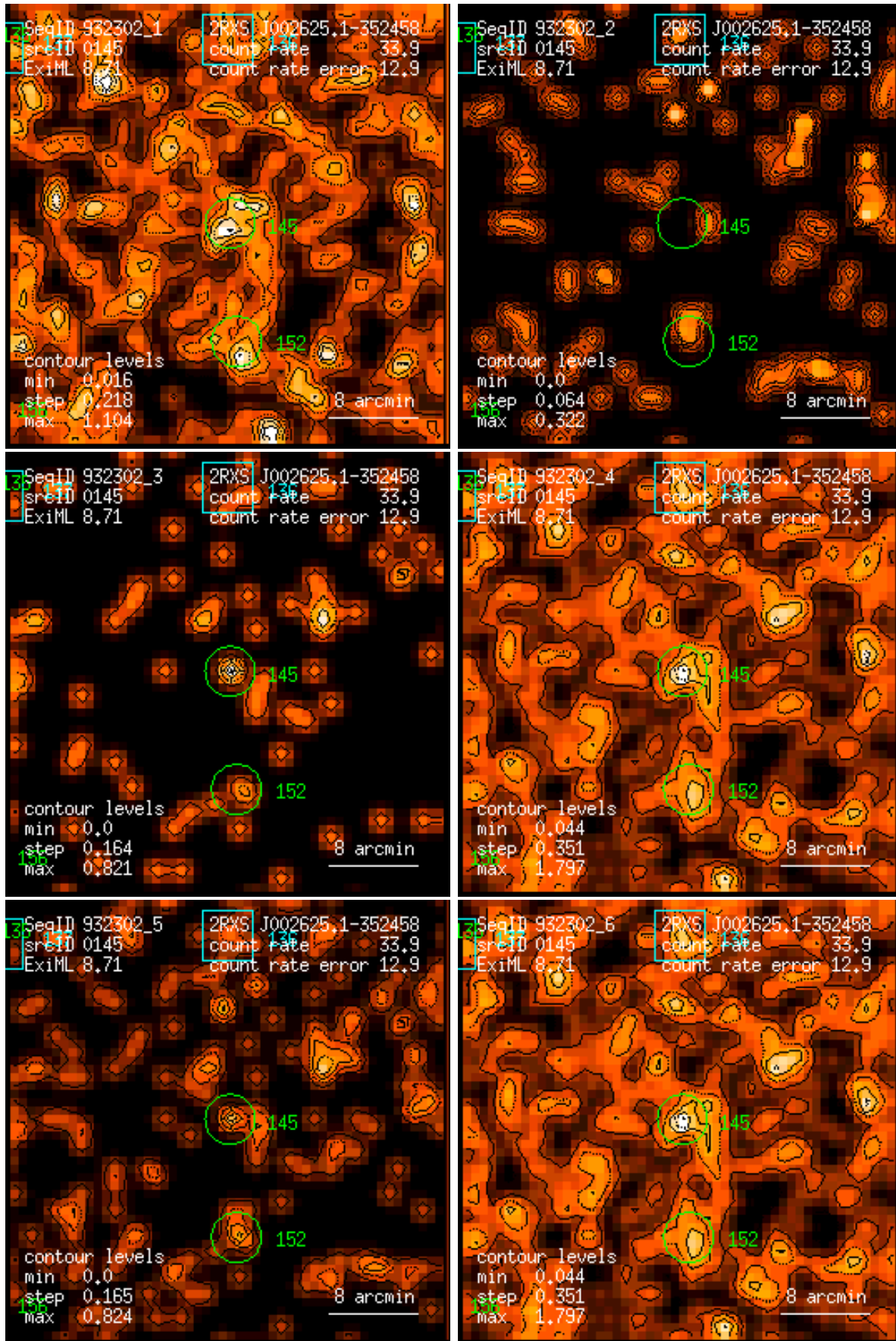
Figure 145: RASS 932302: detection 0145: band rate images, Gaussian filter: (1) PSPC channels 11 – 41, (2) 52 – 90, (3) 91 – 201, (4) 11 – 235, (5) 52 – 201, (6) 11 – 201. Broad band rates in counts/ks. Band rate contour levels in counts/ks/arcmin 2 .
