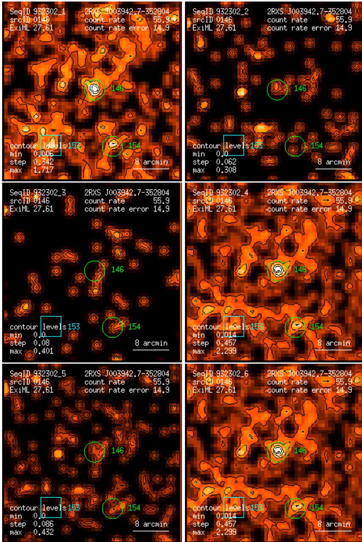
Figure 146: RASS 932302: detection 0146: band rate images, Gaussian filter: (1) PSPC channels 11 – 41, (2) 52 – 90, (3) 91 – 201, (4) 11 – 235, (5) 52 – 201, (6) 11 – 201. Broad band rates in counts/ks. Band rate contour levels in counts/ks/arcmin 2 .
