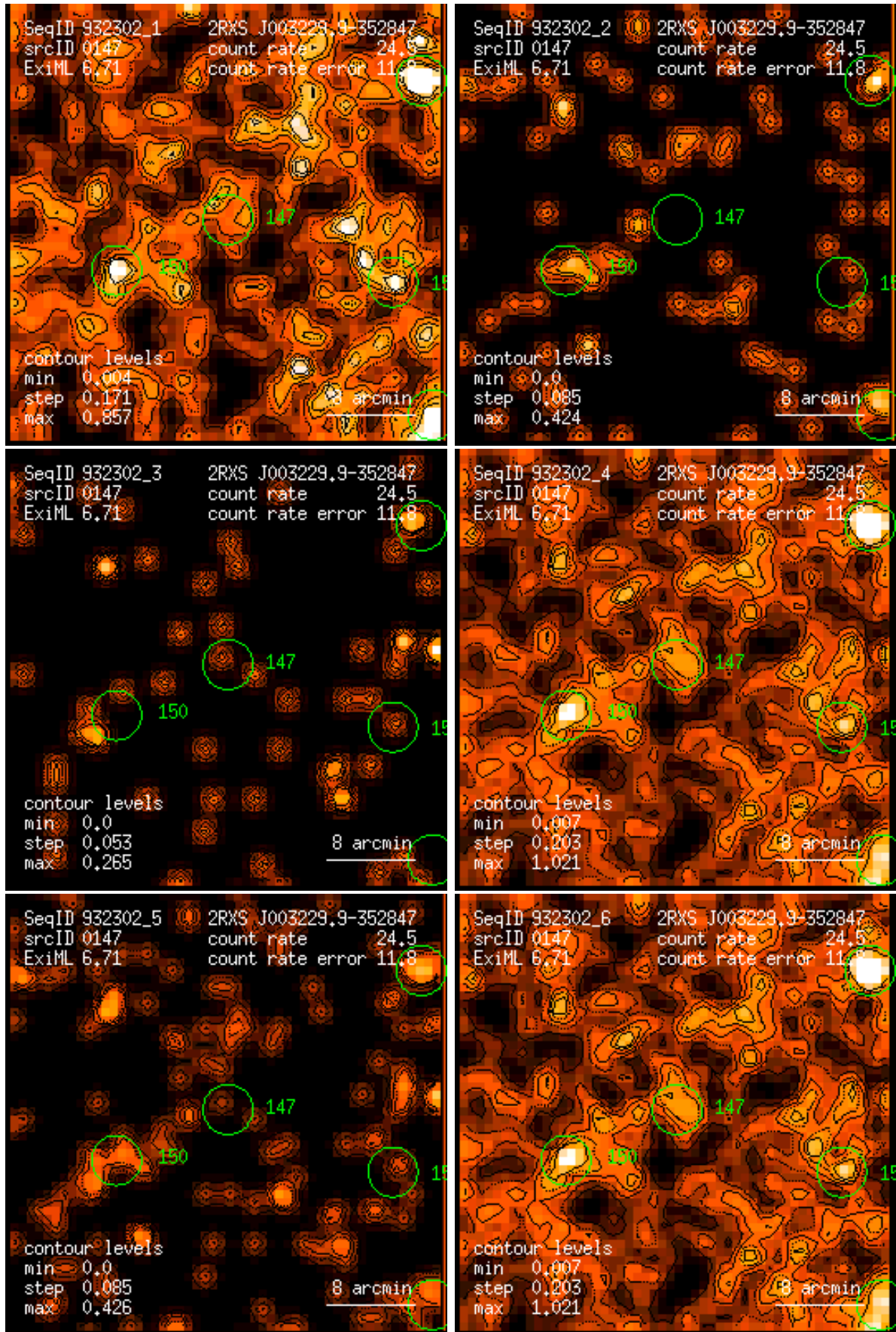
Figure 147: RASS 932302: detection 0147: band rate images, Gaussian filter: (1) PSPC channels 11 – 41, (2) 52 – 90, (3) 91 – 201, (4) 11 – 235, (5) 52 – 201, (6) 11 – 201. Broad band rates in counts/ks. Band rate contour levels in counts/ks/arcmin 2 .
