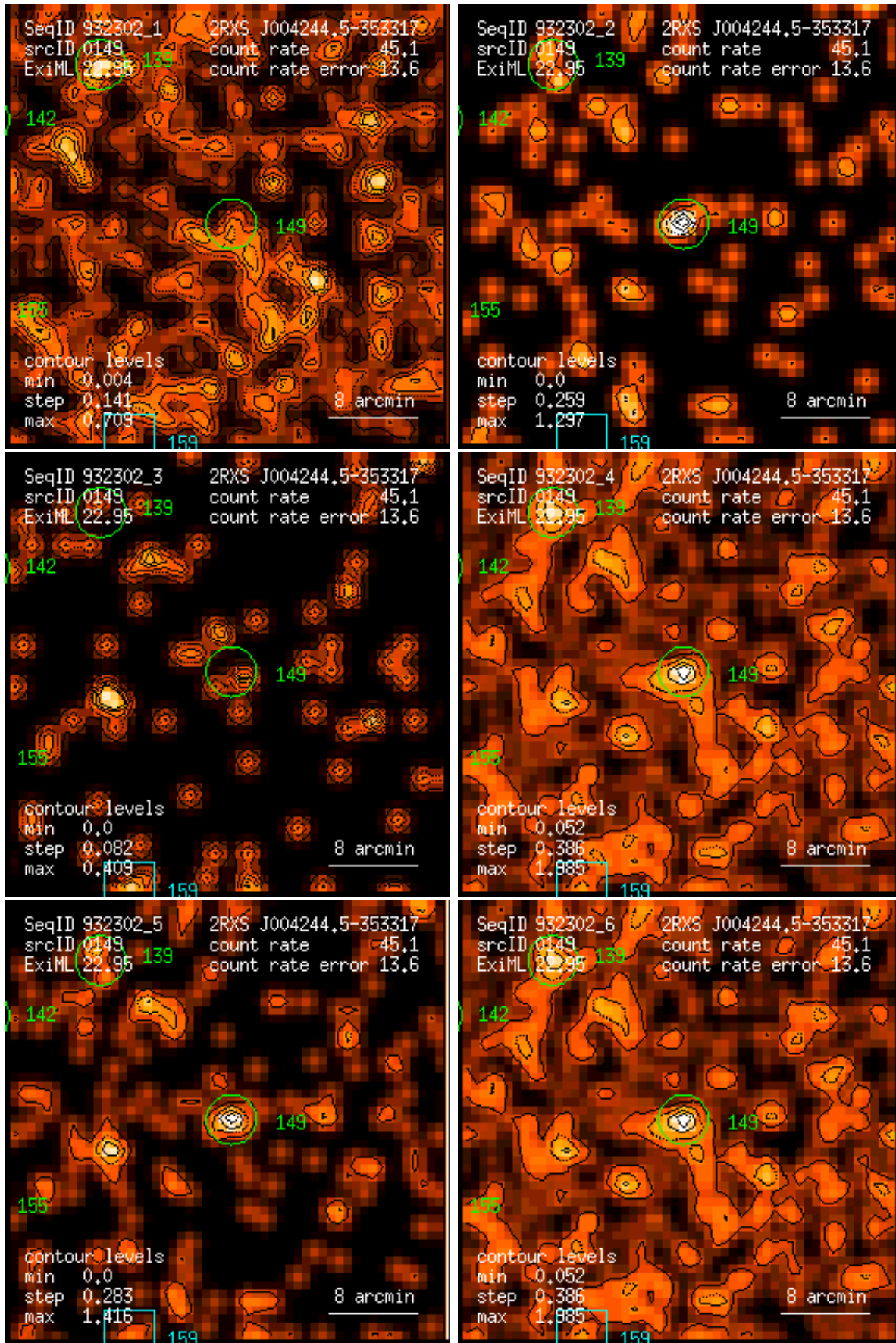
Figure 149: RASS 932302: detection 0149: band rate images, Gaussian filter: (1) PSPC channels 11 – 41, (2) 52 – 90, (3) 91 – 201, (4) 11 – 235, (5) 52 – 201, (6) 11 – 201. Broad band rates in counts/ks. Band rate contour levels in counts/ks/arcmin 2 .
