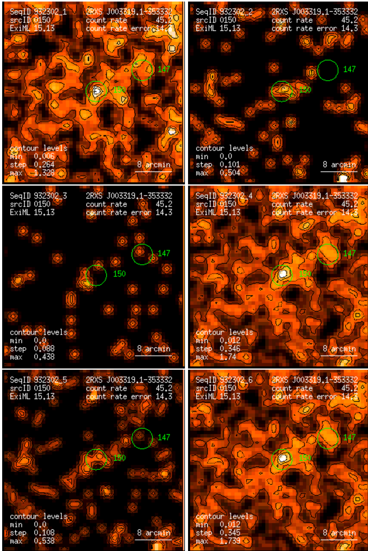
Figure 150: RASS 932302: detection 0150: band rate images, Gaussian filter: (1) PSPC channels 11 – 41, (2) 52 – 90, (3) 91 – 201, (4) 11 – 235, (5) 52 – 201, (6) 11 – 201. Broad band rates in counts/ks. Band rate contour levels in counts/ks/arcmin 2 .
