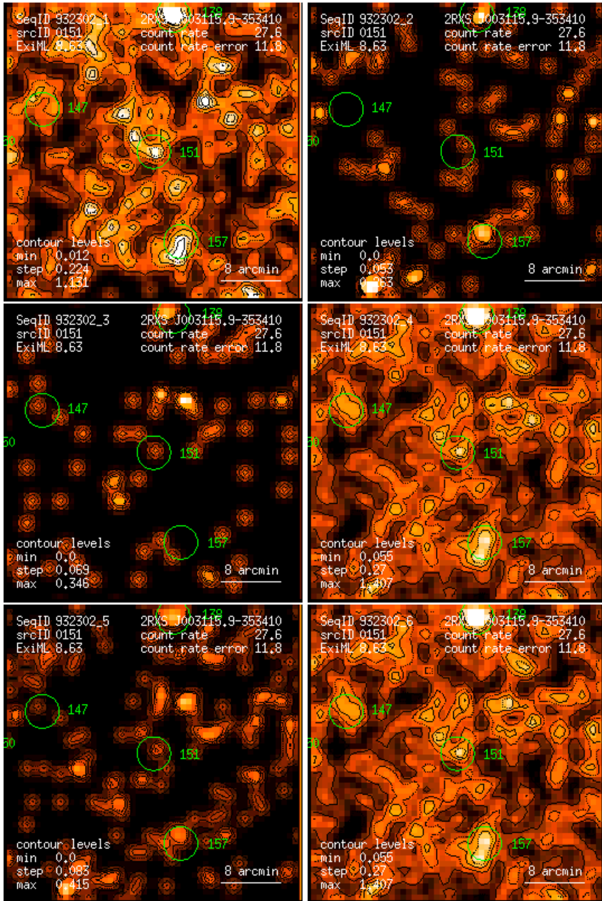
Figure 151: RASS 932302: detection 0151: band rate images, Gaussian filter: (1) PSPC channels 11 – 41, (2) 52 – 90, (3) 91 – 201, (4) 11 – 235, (5) 52 – 201, (6) 11 – 201. Broad band rates in counts/ks. Band rate contour levels in counts/ks/arcmin 2 .
