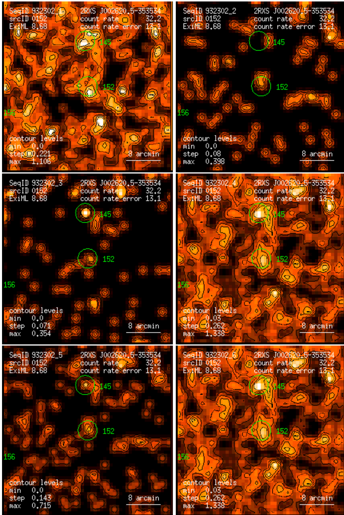
Figure 152: RASS 932302: detection 0152: band rate images, Gaussian filter: (1) PSPC channels 11 – 41, (2) 52 – 90, (3) 91 – 201, (4) 11 – 235, (5) 52 – 201, (6) 11 – 201. Broad band rates in counts/ks. Band rate contour levels in counts/ks/arcmin 2 .
