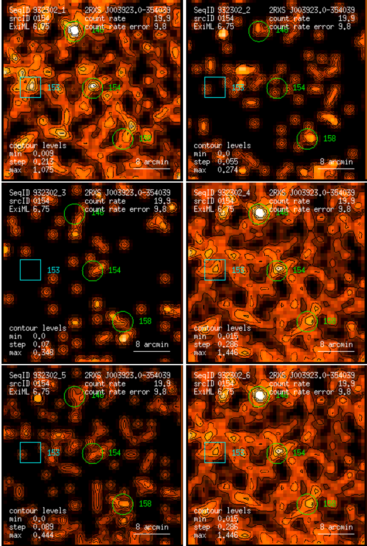
Figure 154: RASS 932302: detection 0154: band rate images, Gaussian filter: (1) PSPC channels 11 – 41, (2) 52 – 90, (3) 91 – 201, (4) 11 – 235, (5) 52 – 201, (6) 11 – 201. Broad band rates in counts/ks. Band rate contour levels in counts/ks/arcmin 2 .
