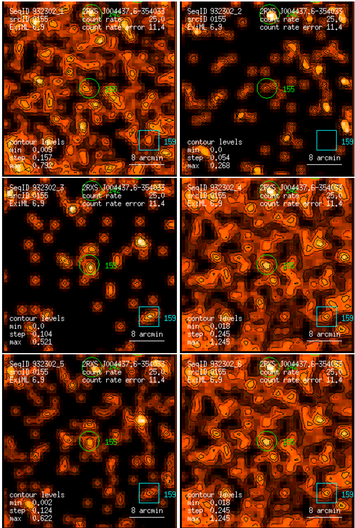
Figure 155: RASS 932302: detection 0155: band rate images, Gaussian filter: (1) PSPC channels 11 – 41, (2) 52 – 90, (3) 91 – 201, (4) 11 – 235, (5) 52 – 201, (6) 11 – 201. Broad band rates in counts/ks. Band rate contour levels in counts/ks/arcmin 2 .
