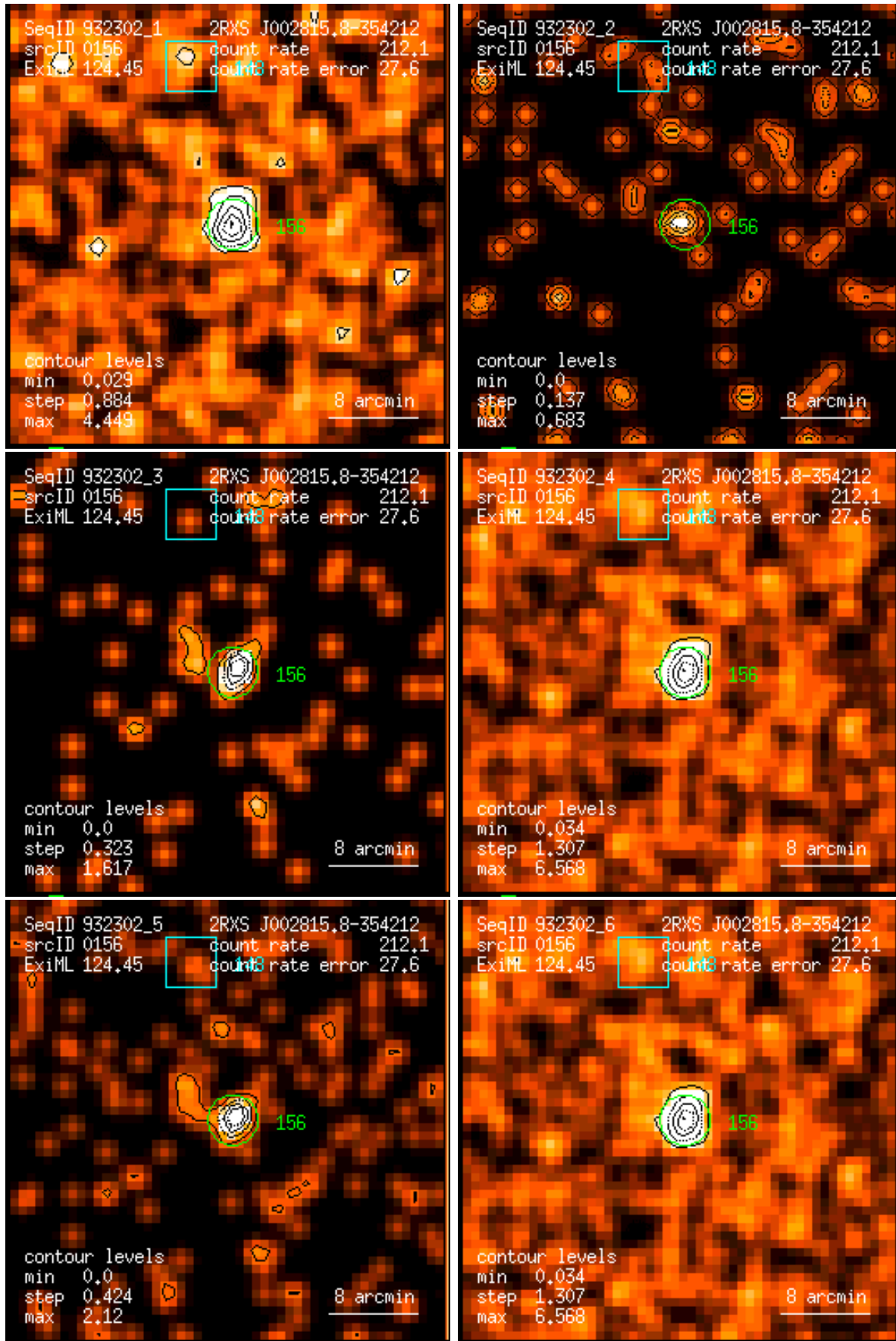
Figure 156: RASS 932302: detection 0156: band rate images, Gaussian filter: (1) PSPC channels 11 – 41, (2) 52 – 90, (3) 91 – 201, (4) 11 – 235, (5) 52 – 201, (6) 11 – 201. Broad band rates in counts/ks. Band rate contour levels in counts/ks/arcmin 2 .
