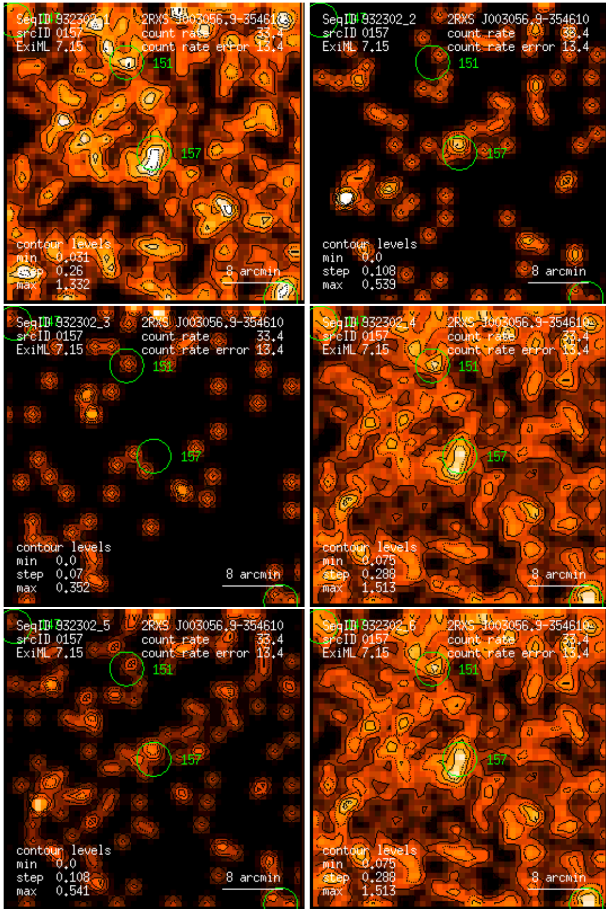
Figure 157: RASS 932302: detection 0157: band rate images, Gaussian filter: (1) PSPC channels 11 – 41, (2) 52 – 90, (3) 91 – 201, (4) 11 – 235, (5) 52 – 201, (6) 11 – 201. Broad band rates in counts/ks. Band rate contour levels in counts/ks/arcmin 2 .
