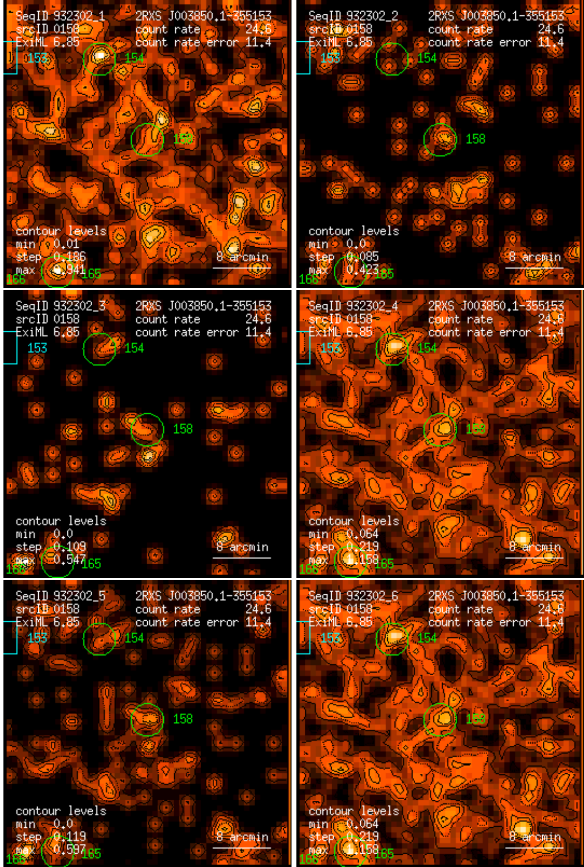
Figure 158: RASS 932302: detection 0158: band rate images, Gaussian filter: (1) PSPC channels 11 – 41, (2) 52 – 90, (3) 91 – 201, (4) 11 – 235, (5) 52 – 201, (6) 11 – 201. Broad band rates in counts/ks. Band rate contour levels in counts/ks/arcmin 2 .
