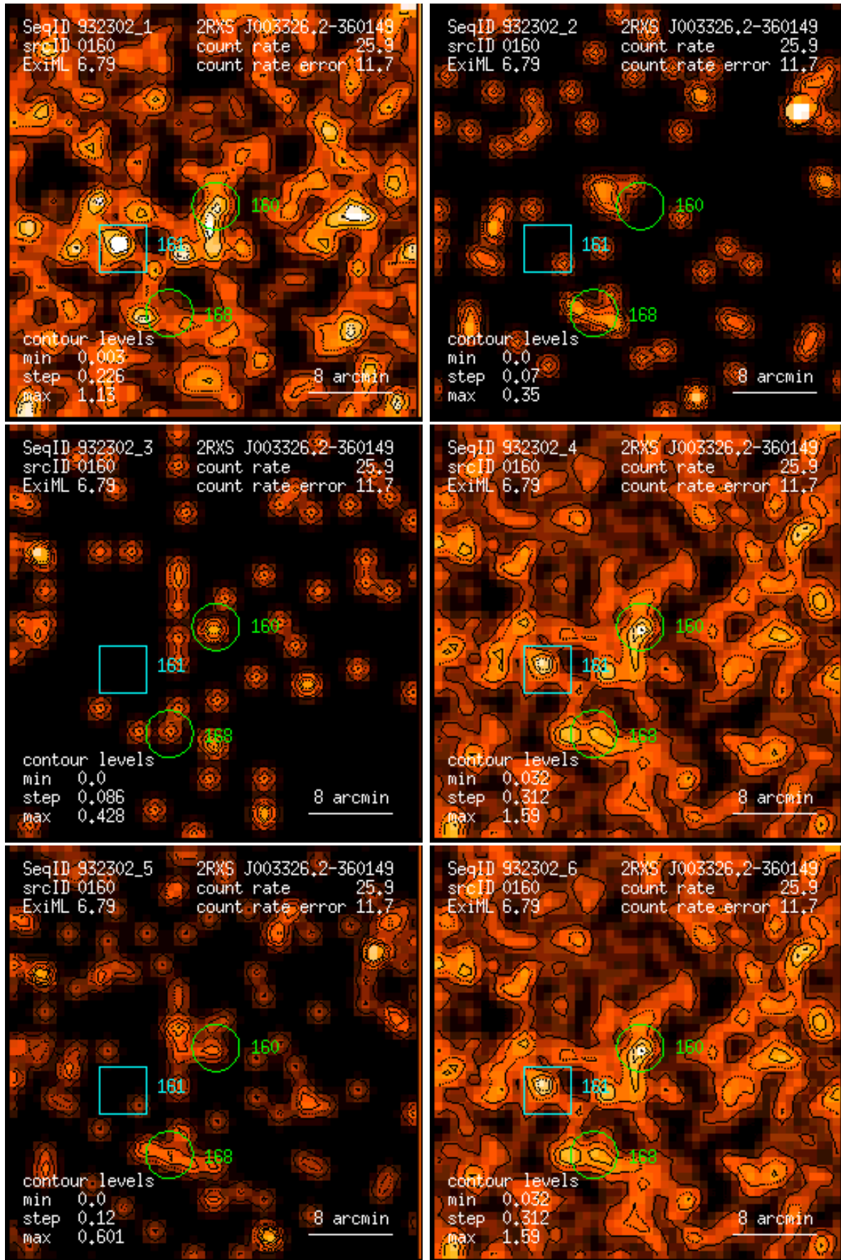
Figure 160: RASS 932302: detection 0160: band rate images, Gaussian filter: (1) PSPC channels 11 – 41, (2) 52 – 90, (3) 91 – 201, (4) 11 – 235, (5) 52 – 201, (6) 11 – 201. Broad band rates in counts/ks. Band rate contour levels in counts/ks/arcmin 2 .
