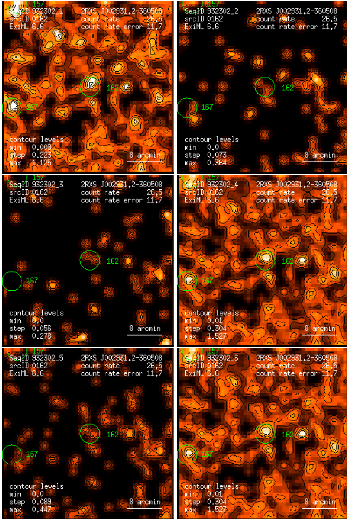
Figure 162: RASS 932302: detection 0162: band rate images, Gaussian filter: (1) PSPC channels 11 – 41, (2) 52 – 90, (3) 91 – 201, (4) 11 – 235, (5) 52 – 201, (6) 11 – 201. Broad band rates in counts/ks. Band rate contour levels in counts/ks/arcmin 2 .
