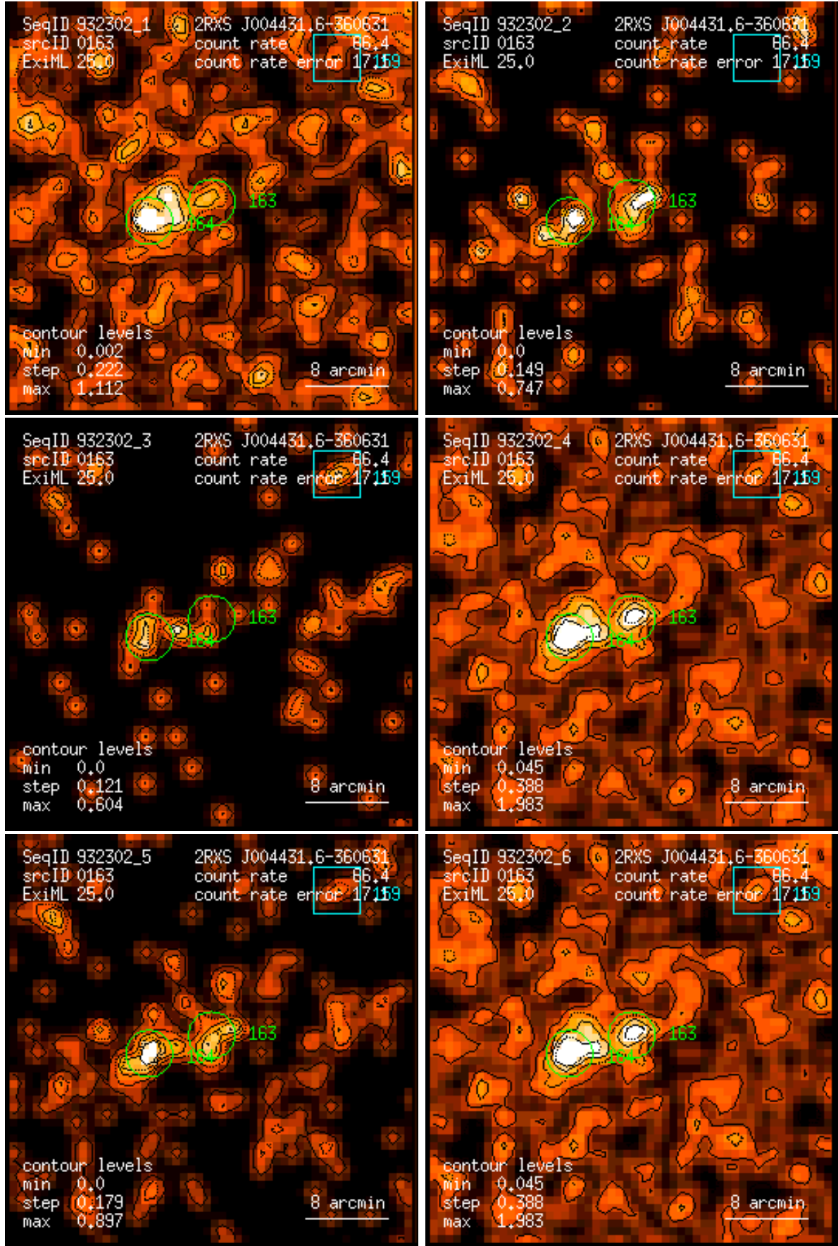
Figure 163: RASS 932302: detection 0163: band rate images, Gaussian filter: (1) PSPC channels 11 – 41, (2) 52 – 90, (3) 91 – 201, (4) 11 – 235, (5) 52 – 201, (6) 11 – 201. Broad band rates in counts/ks. Band rate contour levels in counts/ks/arcmin 2 .
