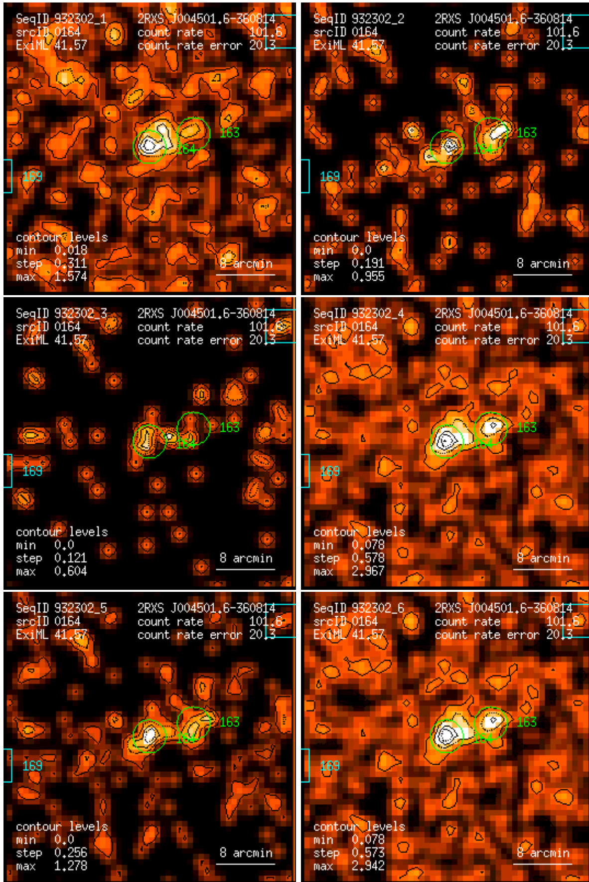
Figure 164: RASS 932302: detection 0164: band rate images, Gaussian filter: (1) PSPC channels 11 – 41, (2) 52 – 90, (3) 91 – 201, (4) 11 – 235, (5) 52 – 201, (6) 11 – 201. Broad band rates in counts/ks. Band rate contour levels in counts/ks/arcmin 2 .
