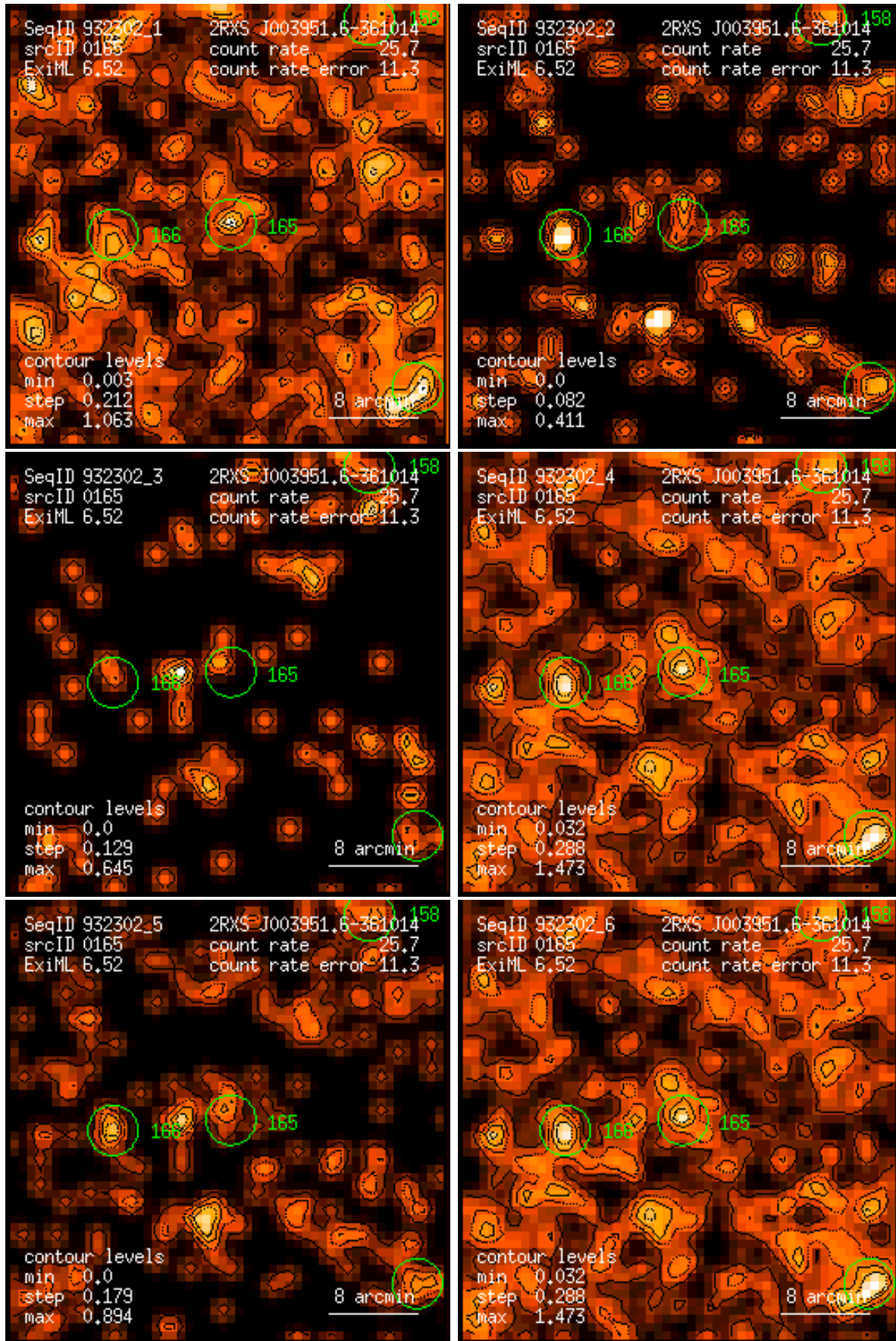
Figure 165: RASS 932302: detection 0165: band rate images, Gaussian filter: (1) PSPC channels 11 – 41, (2) 52 – 90, (3) 91 – 201, (4) 11 – 235, (5) 52 – 201, (6) 11 – 201. Broad band rates in counts/ks. Band rate contour levels in counts/ks/arcmin 2 .
