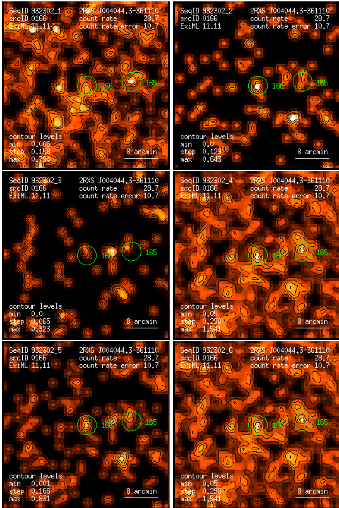
Figure 166: RASS 932302: detection 0166: band rate images, Gaussian filter: (1) PSPC channels 11 – 41, (2) 52 – 90, (3) 91 – 201, (4) 11 – 235, (5) 52 – 201, (6) 11 – 201. Broad band rates in counts/ks. Band rate contour levels in counts/ks/arcmin 2 .
