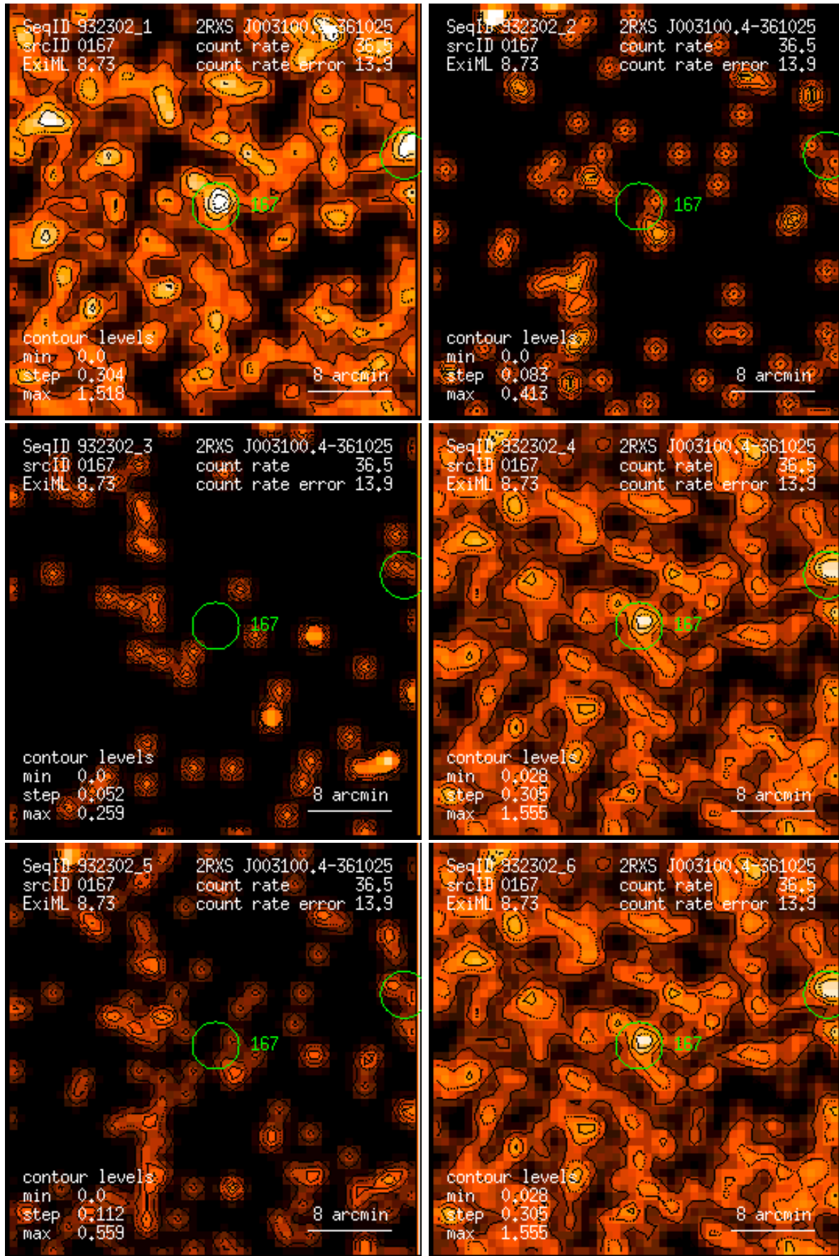
Figure 167: RASS 932302: detection 0167: band rate images, Gaussian filter: (1) PSPC channels 11 – 41, (2) 52 – 90, (3) 91 – 201, (4) 11 – 235, (5) 52 – 201, (6) 11 – 201. Broad band rates in counts/ks. Band rate contour levels in counts/ks/arcmin 2 .
