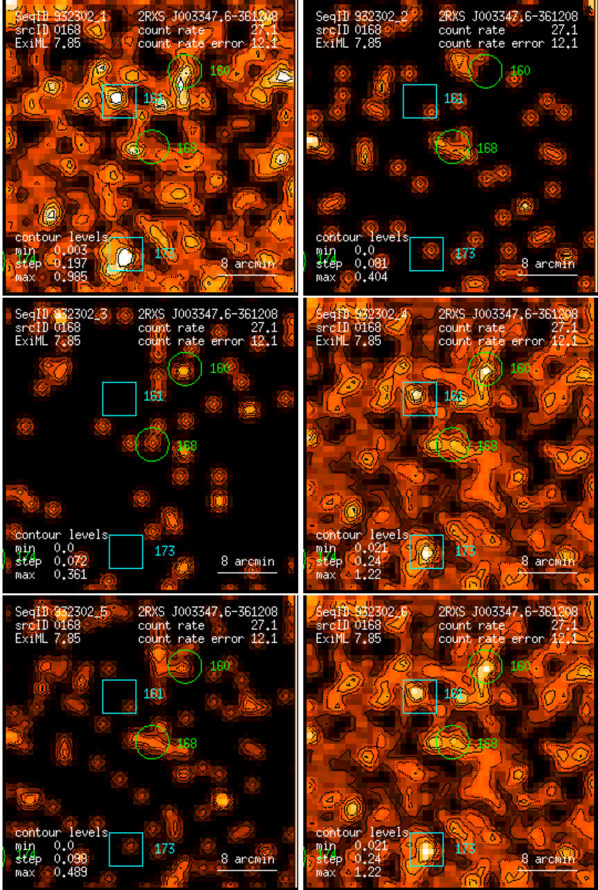
Figure 168: RASS 932302: detection 0168: band rate images, Gaussian filter: (1) PSPC channels 11 – 41, (2) 52 – 90, (3) 91 – 201, (4) 11 – 235, (5) 52 – 201, (6) 11 – 201. Broad band rates in counts/ks. Band rate contour levels in counts/ks/arcmin 2 .
