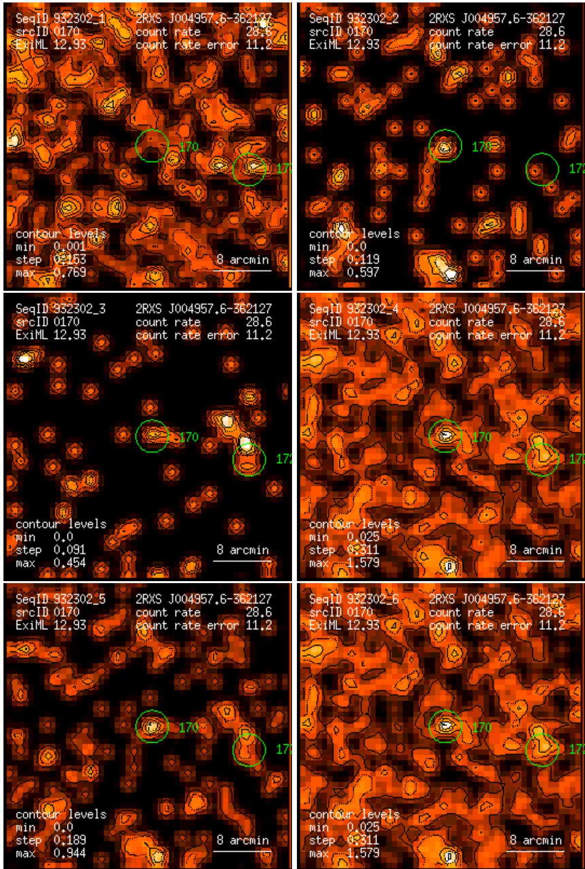
Figure 170: RASS 932302: detection 0170: band rate images, Gaussian filter: (1) PSPC channels 11 – 41, (2) 52 – 90, (3) 91 – 201, (4) 11 – 235, (5) 52 – 201, (6) 11 – 201. Broad band rates in counts/ks. Band rate contour levels in counts/ks/arcmin 2 .
