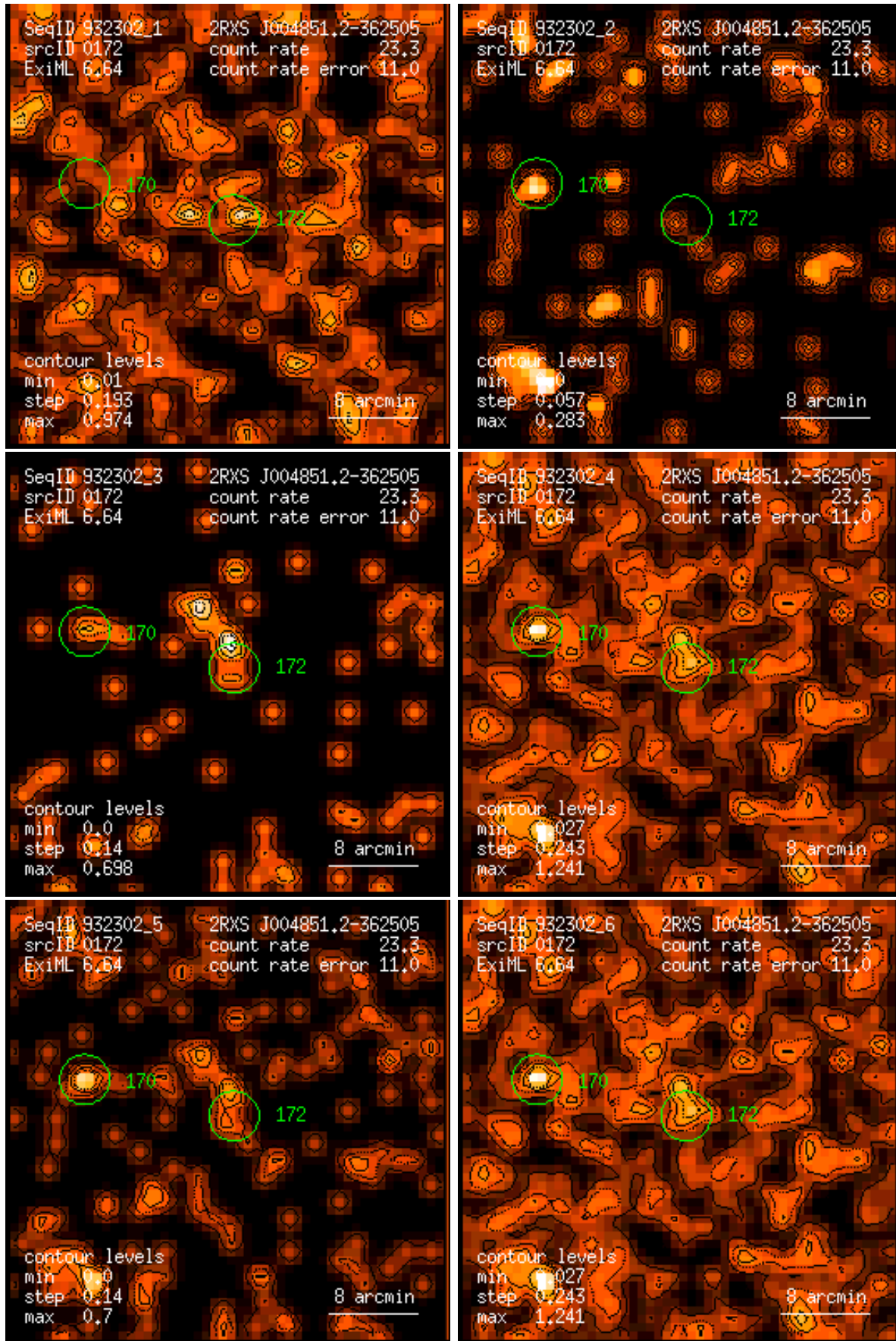
Figure 172: RASS 932302: detection 0172: band rate images, Gaussian filter: (1) PSPC channels 11 – 41, (2) 52 – 90, (3) 91 – 201, (4) 11 – 235, (5) 52 – 201, (6) 11 – 201. Broad band rates in counts/ks. Band rate contour levels in counts/ks/arcmin 2 .
