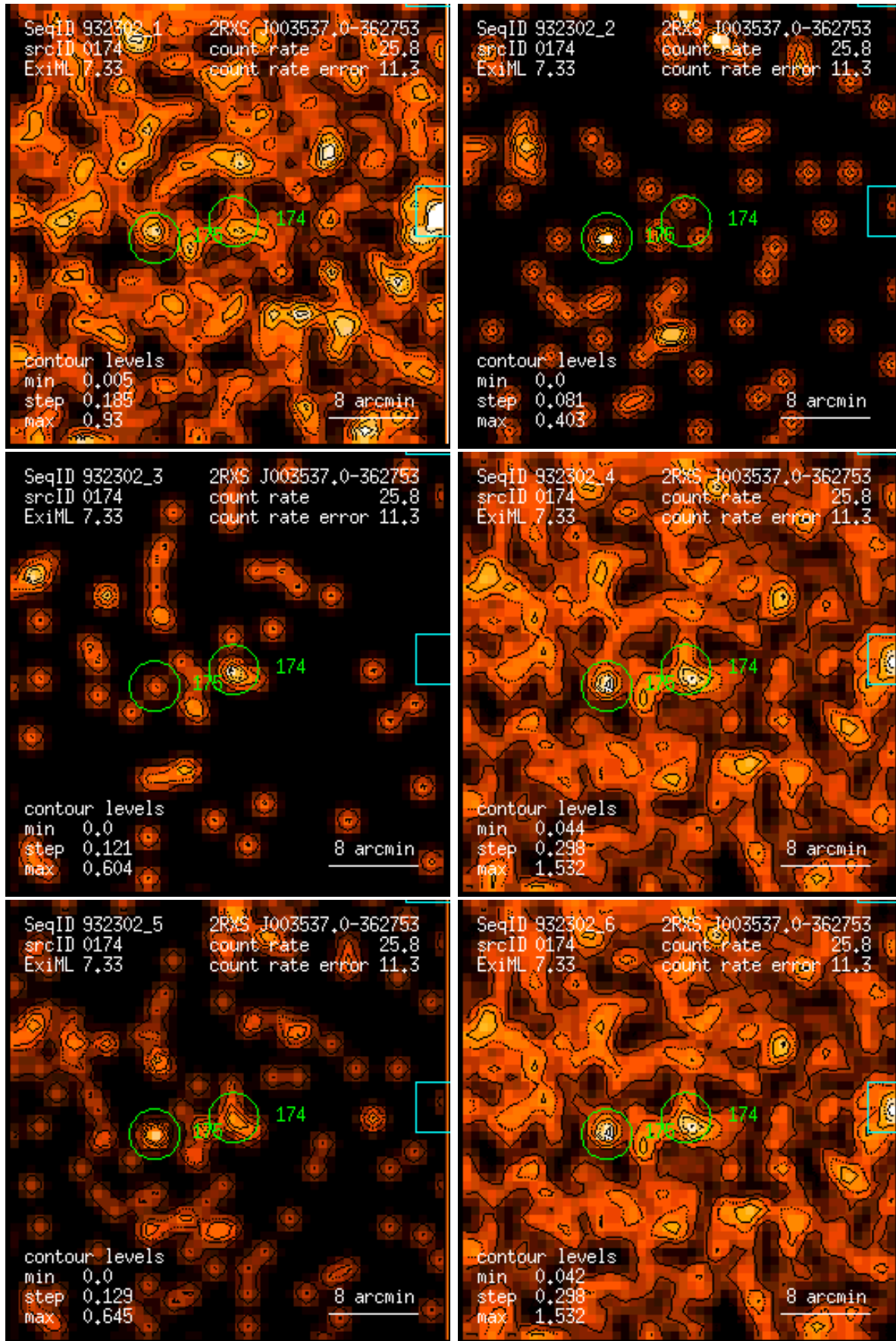
Figure 174: RASS 932302: detection 0174: band rate images, Gaussian filter: (1) PSPC channels 11 – 41, (2) 52 – 90, (3) 91 – 201, (4) 11 – 235, (5) 52 – 201, (6) 11 – 201. Broad band rates in counts/ks. Band rate contour levels in counts/ks/arcmin 2 .
