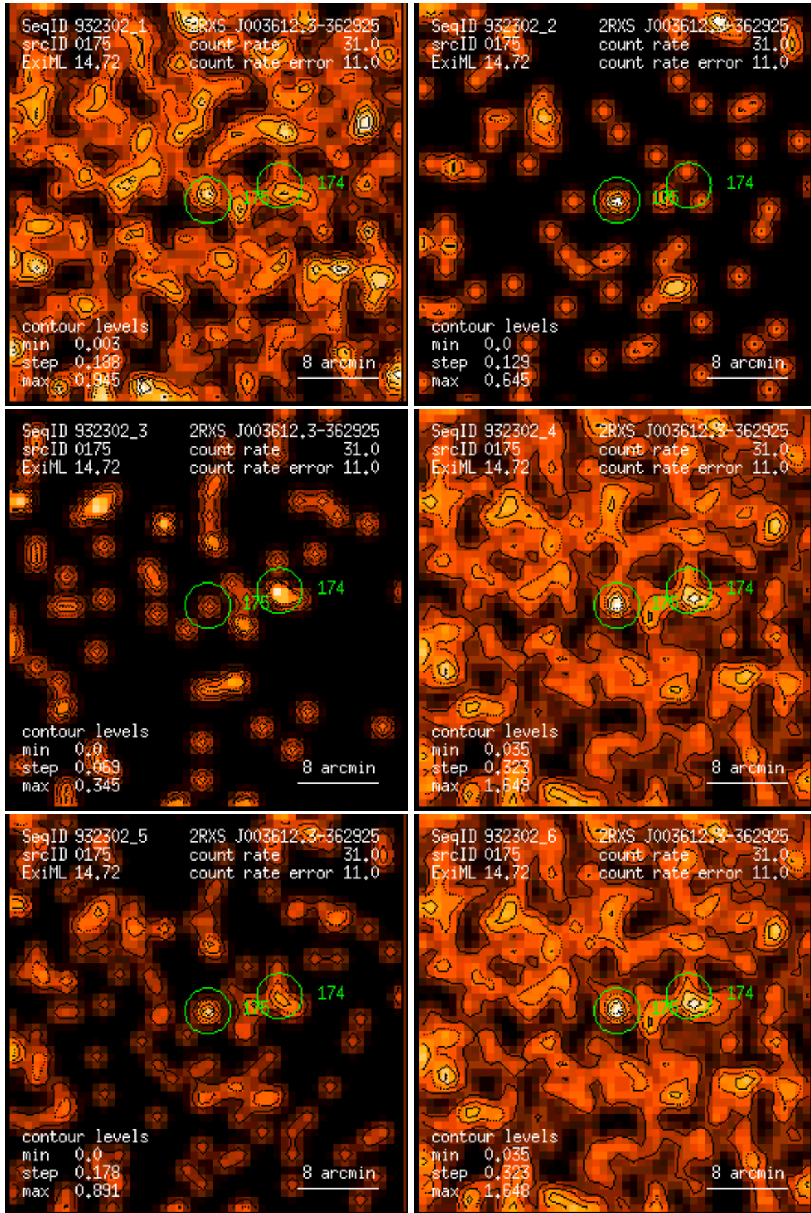
Figure 175: RASS 932302: detection 0175: band rate images, Gaussian filter: (1) PSPC channels 11 – 41, (2) 52 – 90, (3) 91 – 201, (4) 11 – 235, (5) 52 – 201, (6) 11 – 201. Broad band rates in counts/ks. Band rate contour levels in counts/ks/arcmin 2 .
