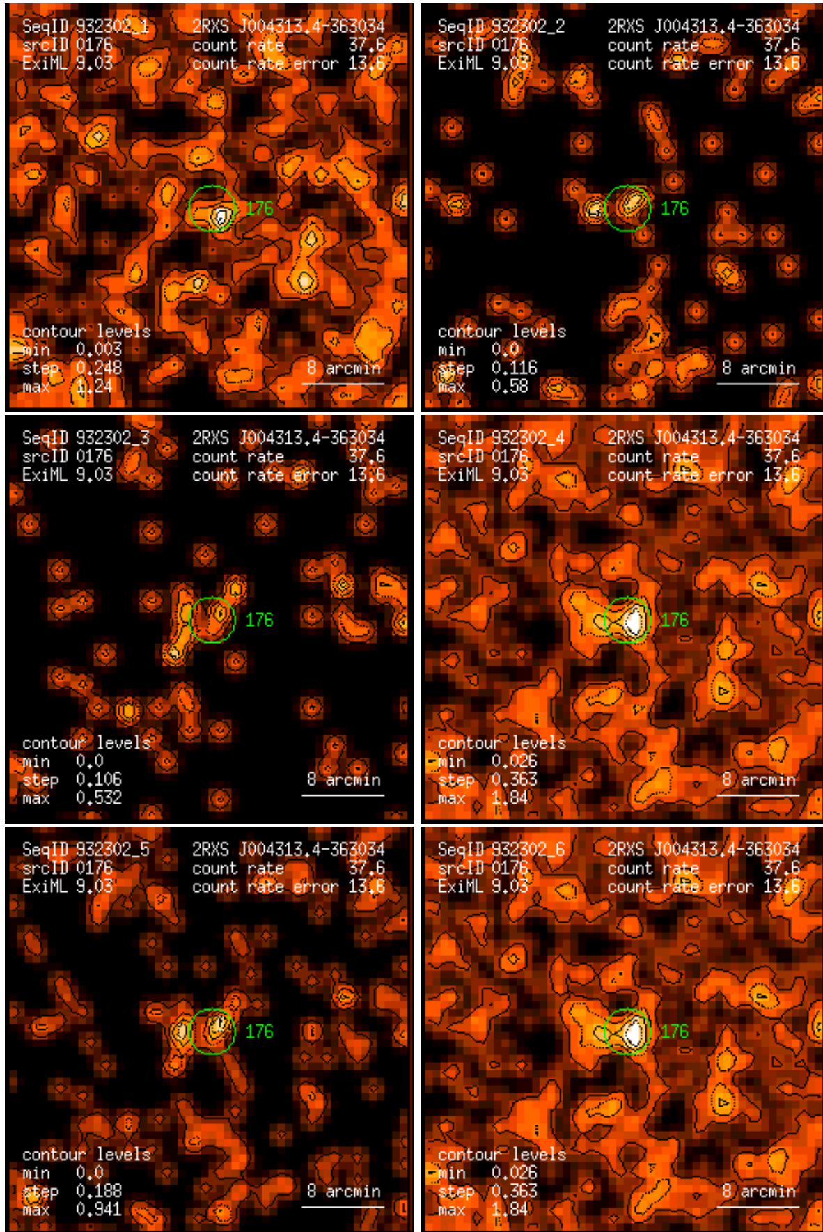
Figure 176: RASS 932302: detection 0176: band rate images, Gaussian filter: (1) PSPC channels 11 – 41, (2) 52 – 90, (3) 91 – 201, (4) 11 – 235, (5) 52 – 201, (6) 11 – 201. Broad band rates in counts/ks. Band rate contour levels in counts/ks/arcmin 2 .
