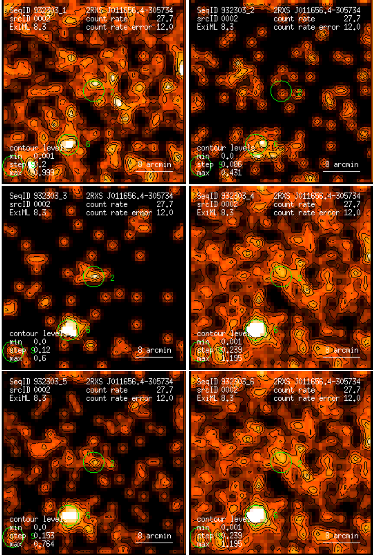
Figure 2: RASS 932303: detection 0002: band rate images, Gaussian filter: (1) PSPC channels 11 – 41, (2) 52 – 90, (3) 91 – 201, (4) 11 – 235, (5) 52 – 201, (6) 11 – 201. Broad band rates in counts/ks. Band rate contour levels in counts/ks/arcmin 2 .
